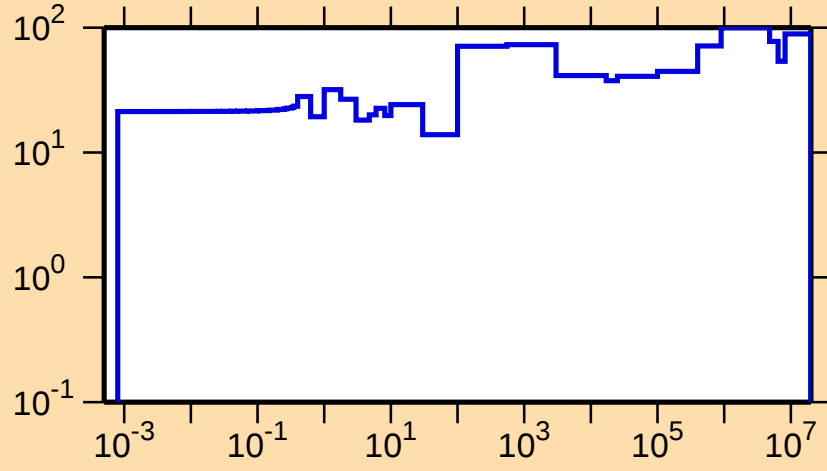
\Delta\sigma/\sigma vs. E for ^{128}\text{I}(n,\gamma)
