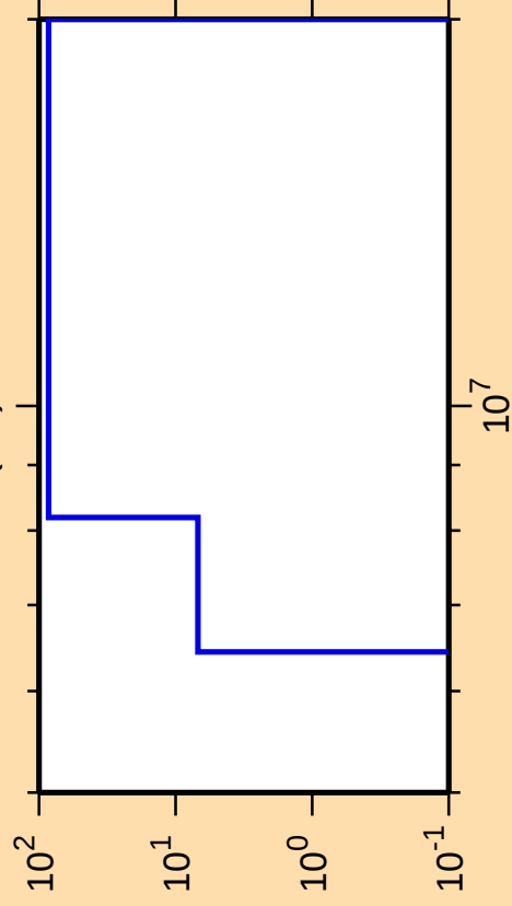
\Delta\sigma/\sigma vs. E for ^{128}\text{I}(n,t)
