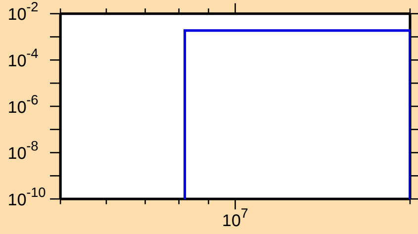
\sigma vs. E for ^{128}\text{I}(n,np)
