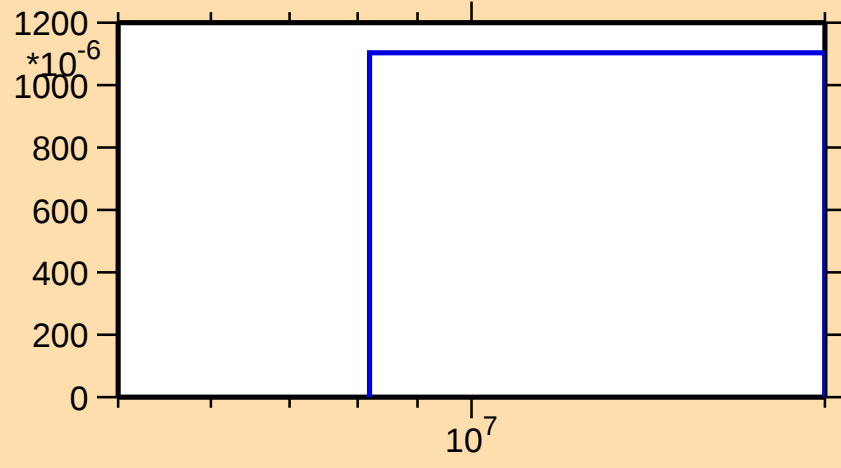
\sigma vs. E for ^{128}\text{I}(n,3n)
