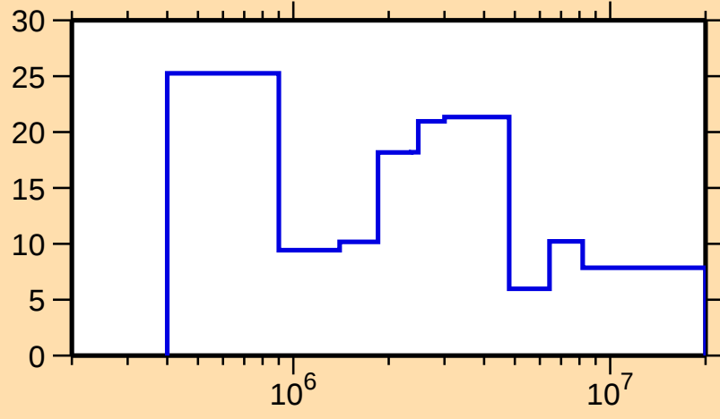
\Delta\sigma/\sigma vs. E for ^{128}\text{I}(\text{n},\text{el.})
