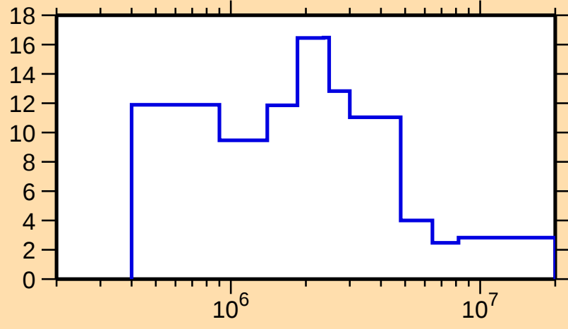
\Delta\sigma/\sigma vs. E for ^{128}\text{I}(\text{n},\text{tot.})
