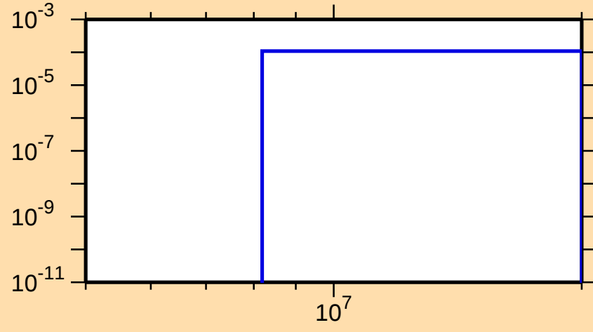
\sigma vs. E for ^{128}\text{I}(n,t)
