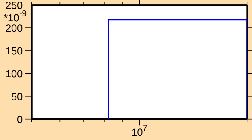
\sigma vs. E for ^{128}\text{I}(n,2np)
