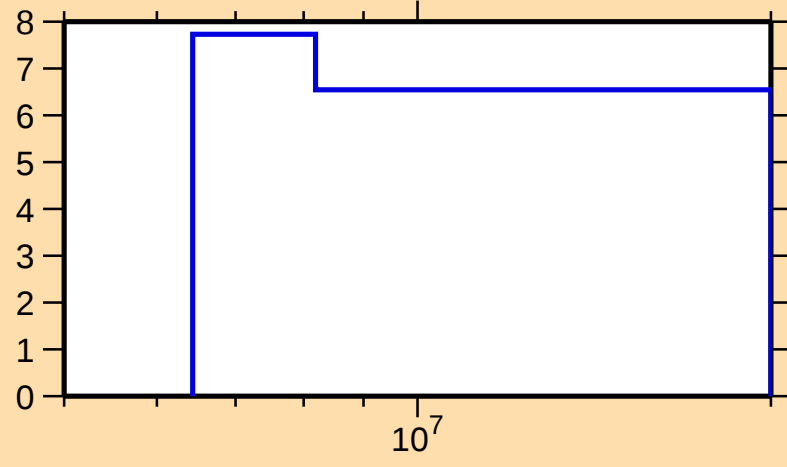
\Delta\sigma/\sigma vs. E for ^{128}\text{I}(n,\text{nonel.})
