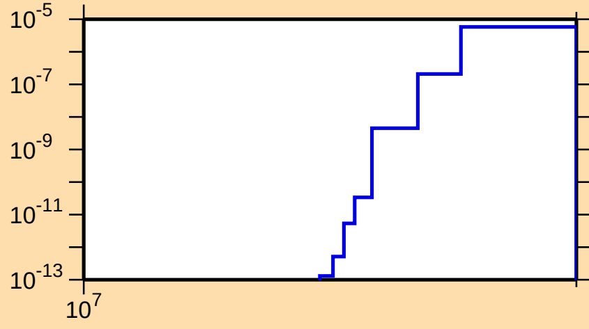
\sigma vs. E for ^{134}\text{I}(n,\text{nd})
