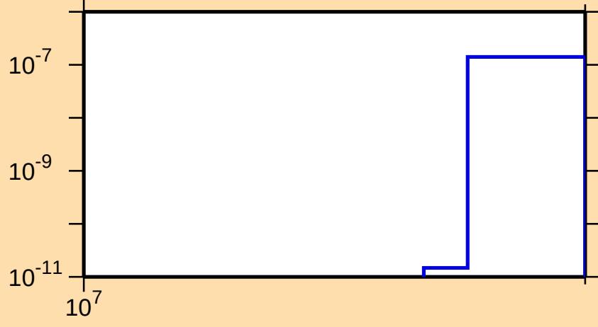
\sigma vs. E for ^{134}\text{I}(n,\text{nt})
