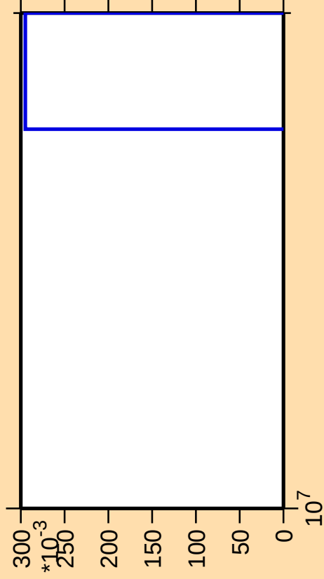
\Delta\sigma/\sigma vs. E for ^{137}\text{I} (mt 42)
