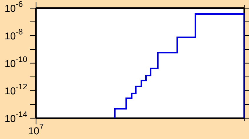
\sigma vs. E for ^{137}\text{I}(n,2n\alpha)
