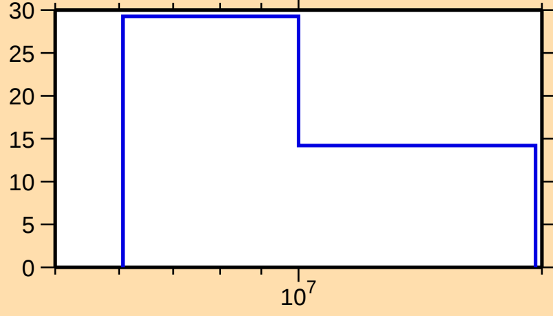
\Delta\sigma/\sigma vs. E for ^{137}\text{I}(n,\text{el.})
