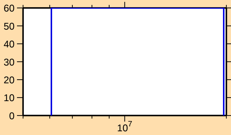
\Delta\sigma/\sigma vs. E for ^{137}\text{I}(n,n\text{cont.})
