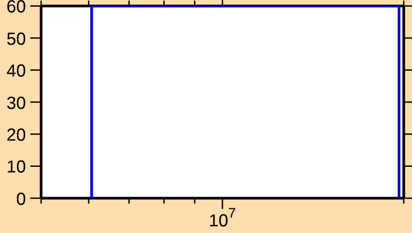
\Delta\sigma/\sigma vs. E for ^{137}\text{I}(\text{n,inel.})
