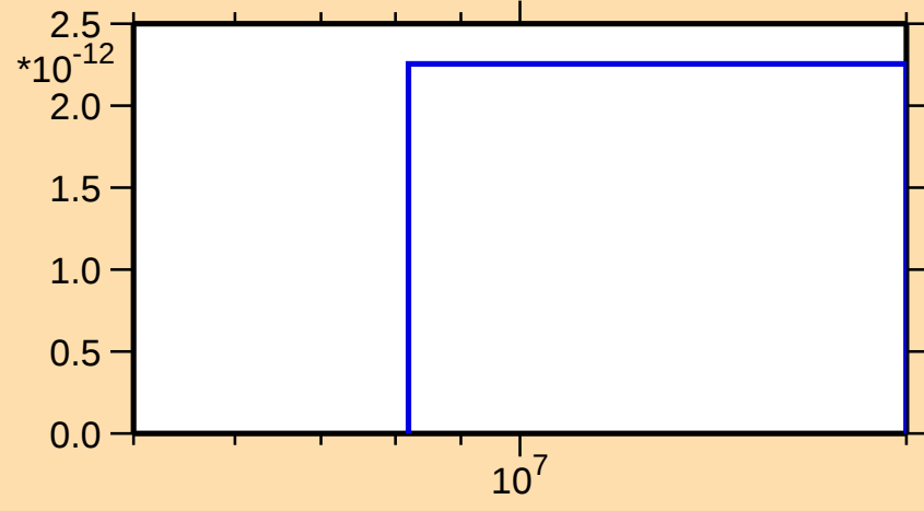
\sigma vs. E for ^{137}\text{I}(\text{mt } 11)
