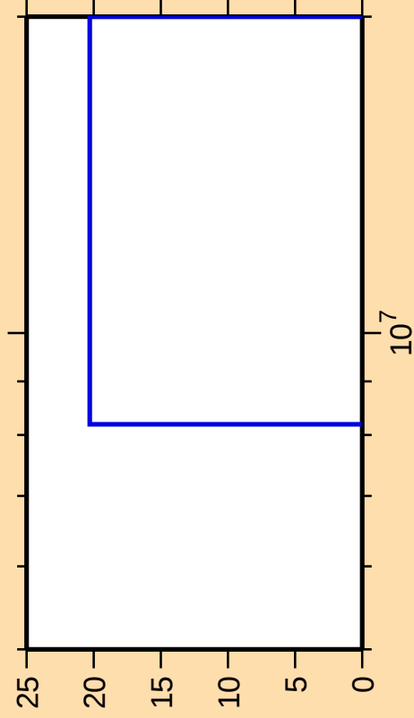
\Delta\sigma/\sigma vs. E for ^{137}\text{I}(\text{mt } 11)
