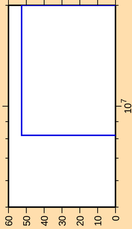
\Delta\sigma/\sigma vs. E for ^{137}\text{I}(n,3n)
