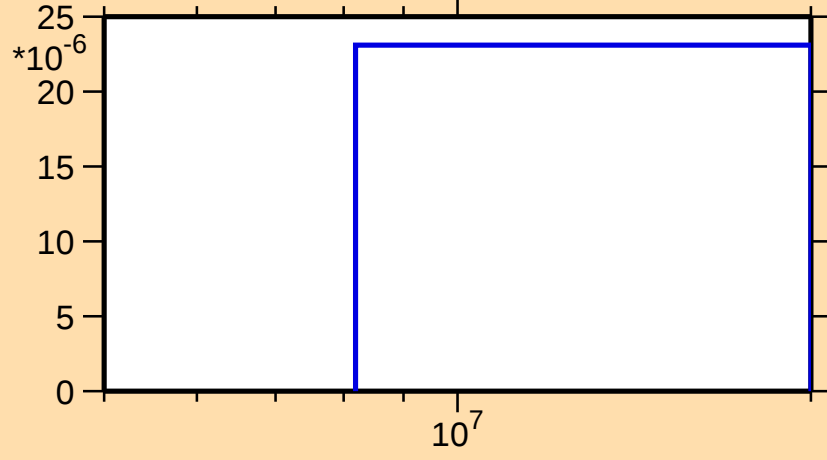
\sigma vs. E for ^{137}\text{I}(n,np)
