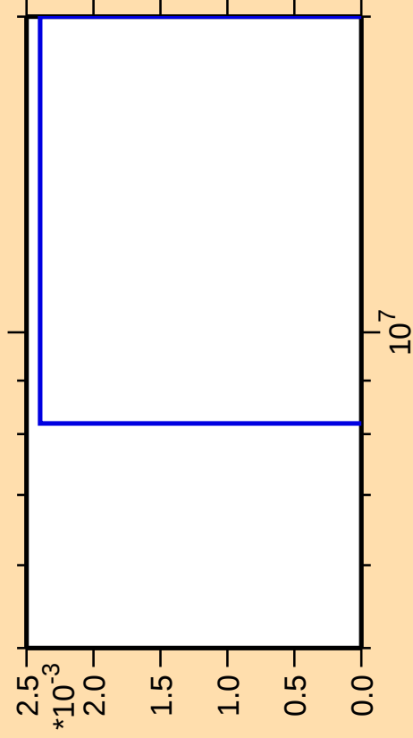
\Delta\sigma/\sigma vs. E for ^{137}\text{I}(\text{mt } 42)
