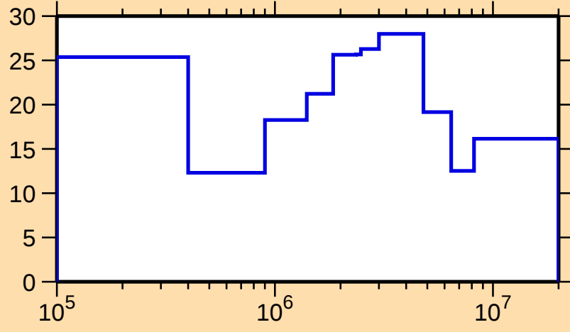
\Delta\sigma/\sigma vs. E for ^{137}\text{I}(\text{n,tot.})
