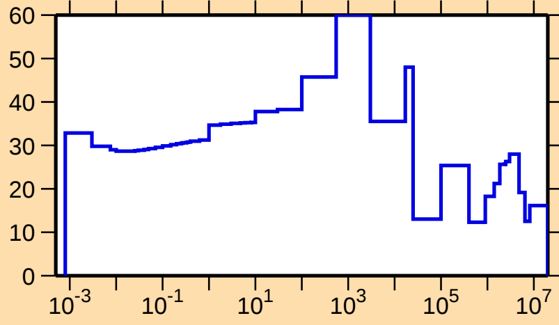
\Delta\sigma/\sigma vs. E for ^{137}\text{I}(n,\text{tot.})
