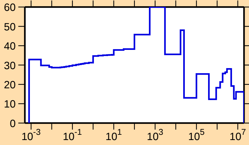
\Delta\sigma/\sigma vs. E for ^{137}\text{I}(n,\text{tot.})
