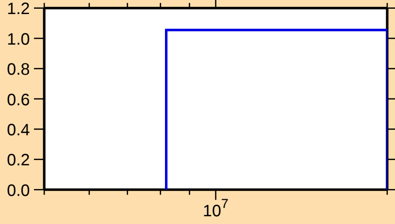
\sigma vs. E for ^{137}\text{I}(n,3n)
