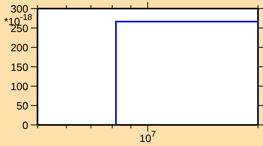
\sigma vs. E for ^{137}\text{I}(\text{mt } 42)
