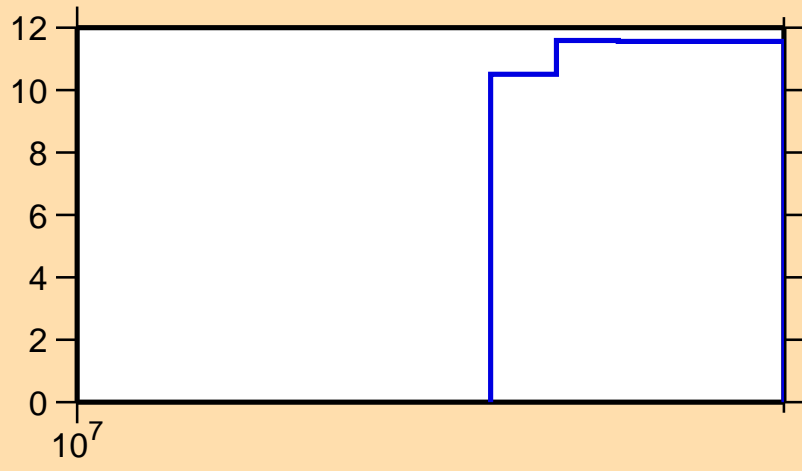
\Delta\sigma/\sigma vs. E for ^{99}\text{In}(n,\text{nonel.})
