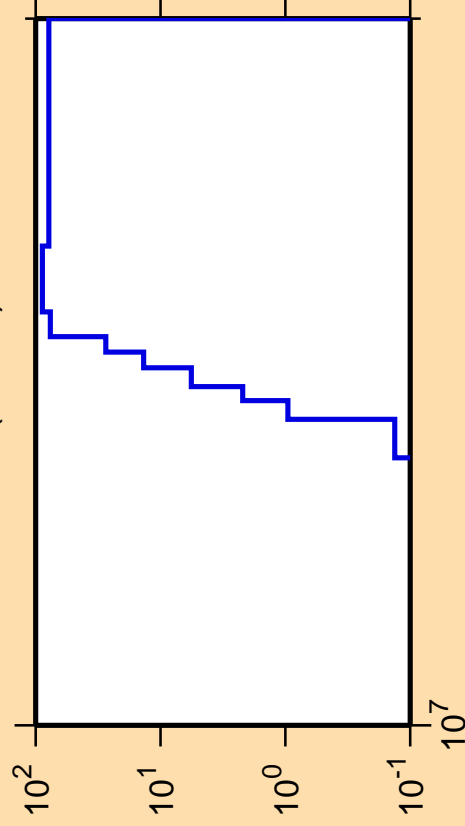
\Delta\sigma/\sigma vs. E for ^{99}\text{In} (mt 45)
