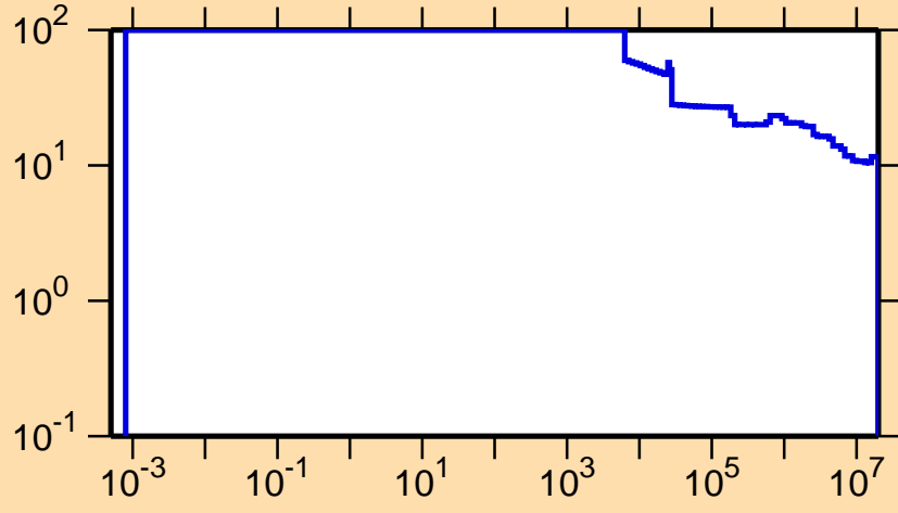
\Delta\sigma/\sigma vs. E for ^{99}\text{In}(n,\text{nonel.})
