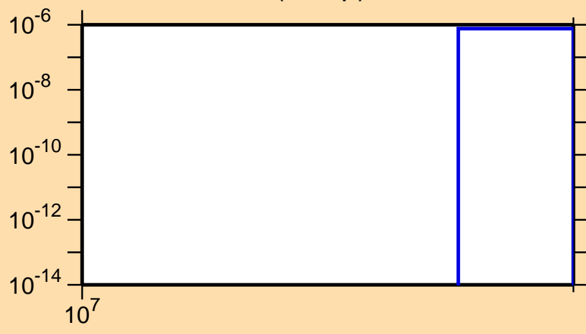
\sigma vs. E for ^{99}\text{In}(n,2np)
