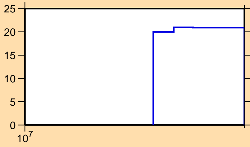
\Delta\sigma/\sigma vs. E for ^{99}\text{In}(n,\text{tot.})
