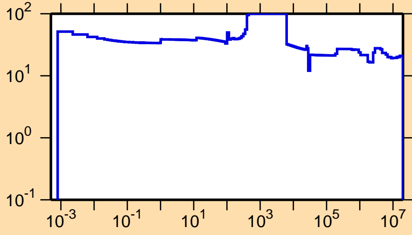
\Delta\sigma/\sigma vs. E for ^{99}\text{In}(n,\text{tot.})
