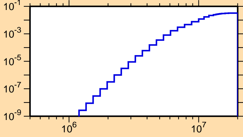
\sigma vs. E for ^{99}\text{In}(n,d)
