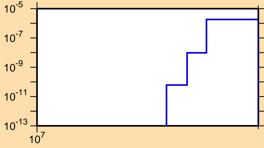
\sigma vs. E for ^{99}\text{In}(n,\text{pt})
