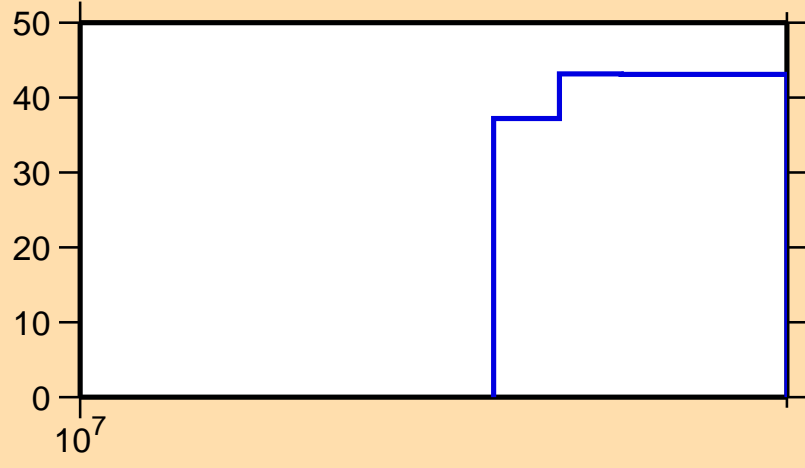
\Delta\sigma/\sigma vs. E for ^{99}\text{In}(n,\text{el.})
