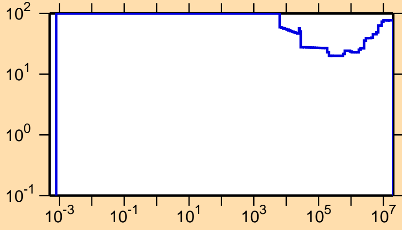
\Delta\sigma/\sigma vs. E for ^{99}\text{In}(n,p)
