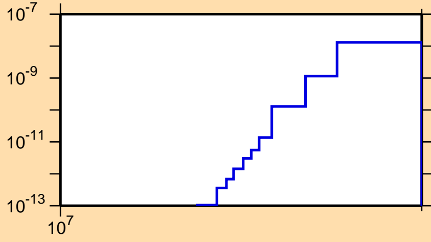
\sigma vs. E for ^{99}\text{In}(\text{mt117})
