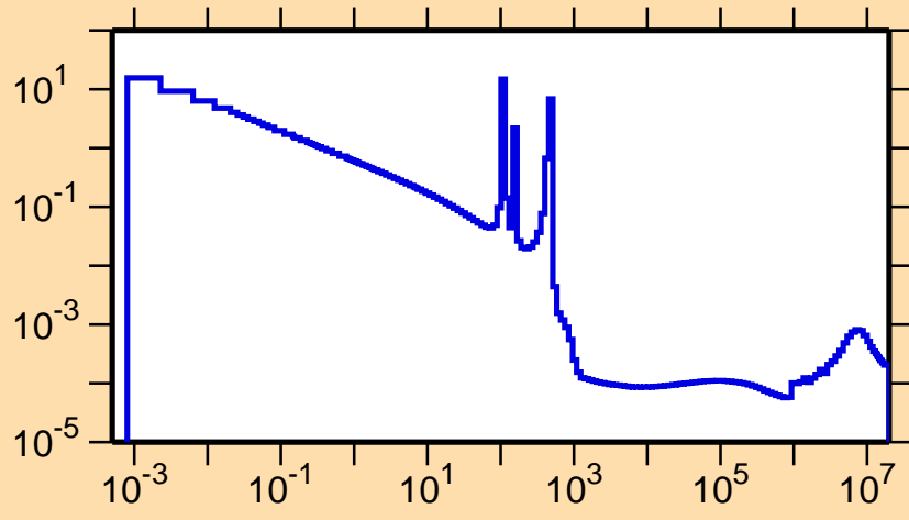
\sigma vs. E for ^{99}\text{In}(n,\gamma)
