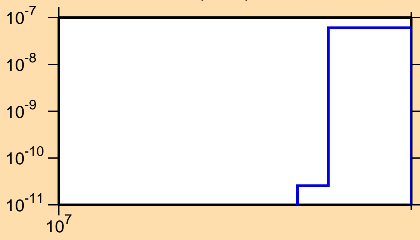
\sigma vs. E for ^{99}\text{In}(n,nd)
