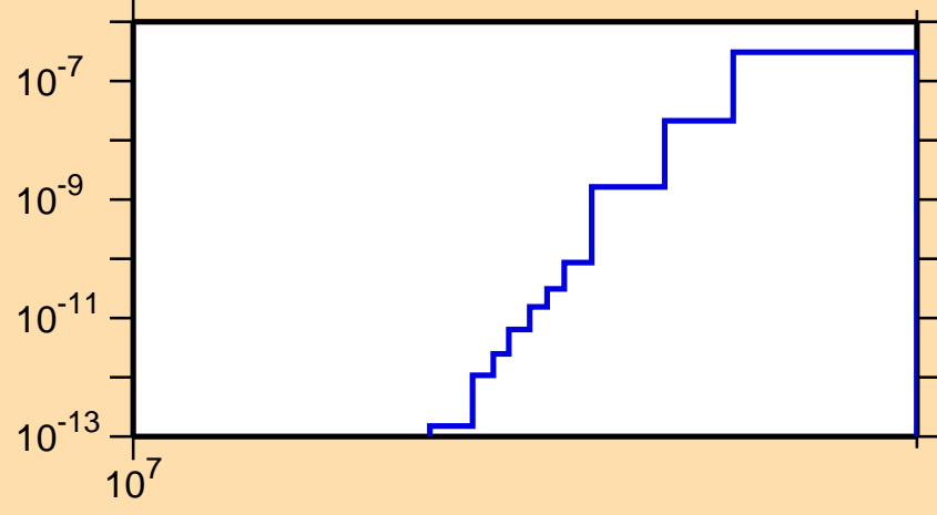
\sigma vs. E for ^{99}\text{In} (mt 45)
