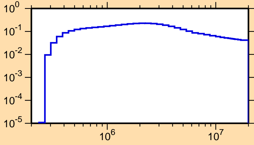
\sigma vs. E for ^{99}\text{In}(n,\text{inel.})
