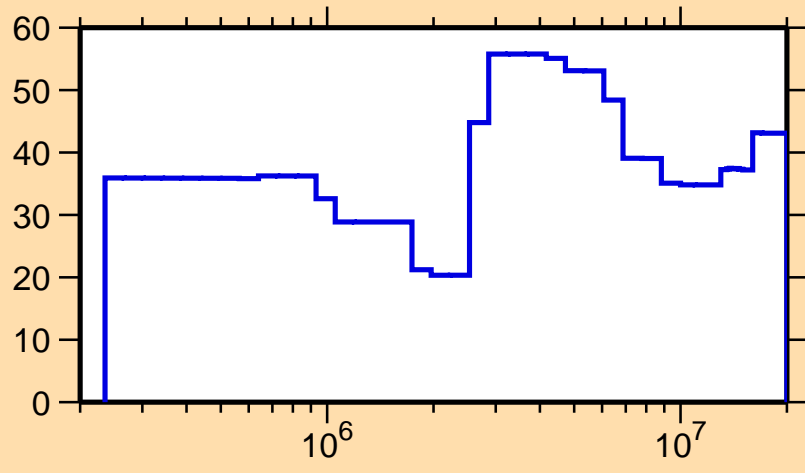
\Delta\sigma/\sigma vs. E for ^{99}\text{In}(n,\text{el.})
