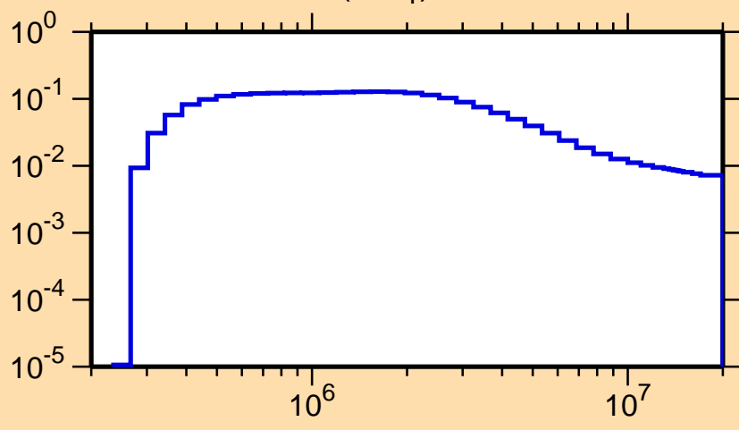
\sigma vs. E for ^{99}\text{In}(n,n_1)
