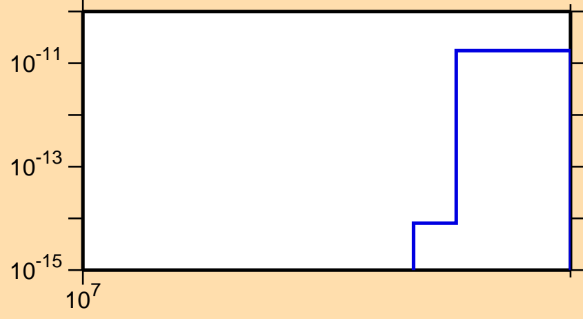
\sigma vs. E for ^{99}\text{In} (mt 34)
