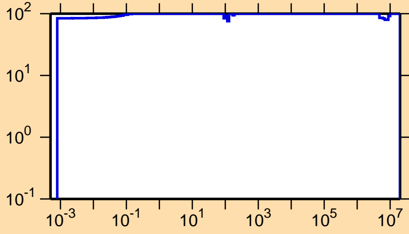
\Delta\sigma/\sigma vs. E for ^{99}\text{In}(n,\gamma)
