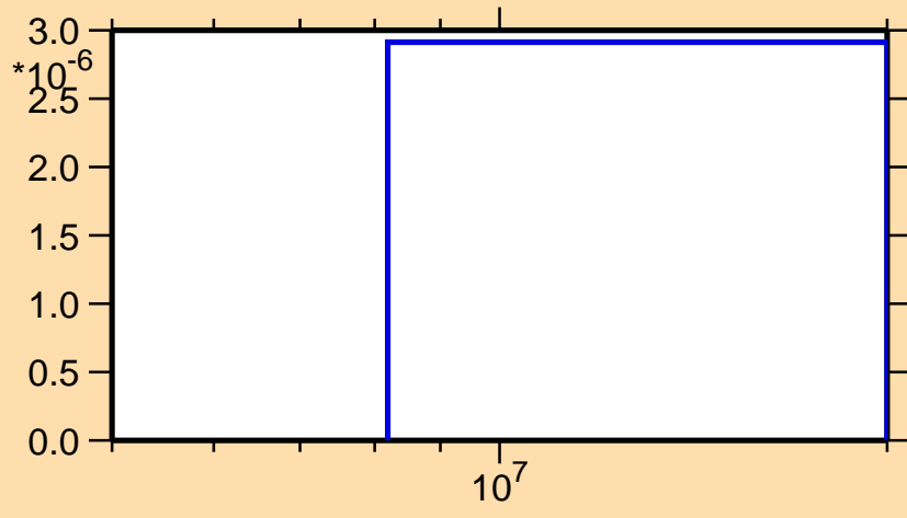
\sigma vs. E for ^{99}\text{In}(n,n\alpha)
