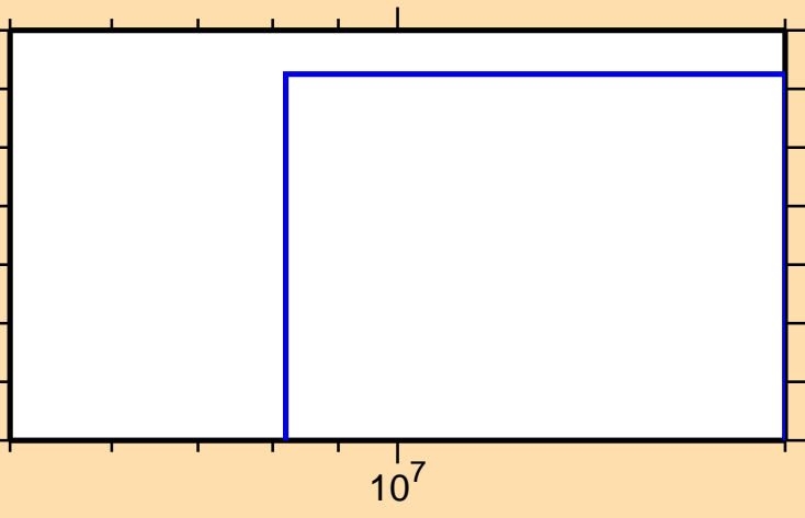
\sigma vs. E for ^{99}\text{In}(n,2n)
