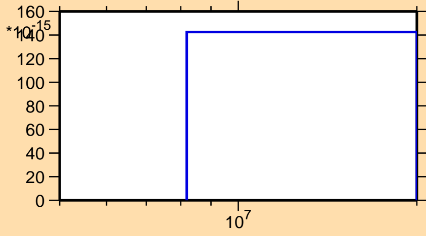
\sigma vs. E for ^{99}\text{In}(\text{mt } 34)
