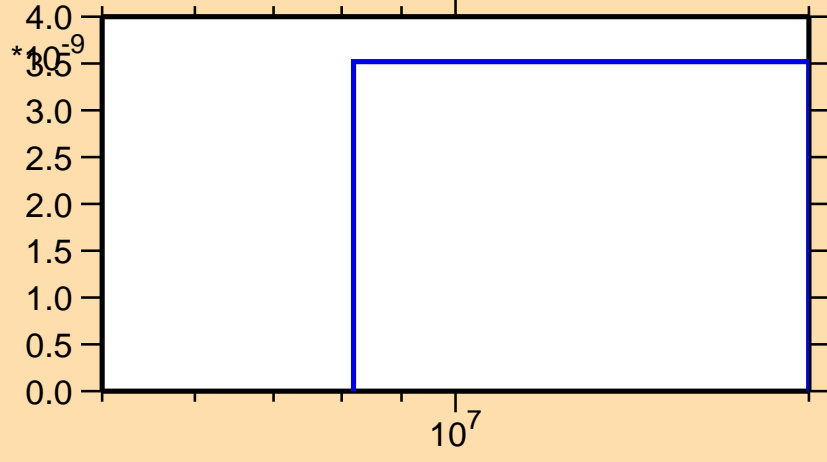
\sigma vs. E for ^{99}\text{In}(\text{mt } 45)
