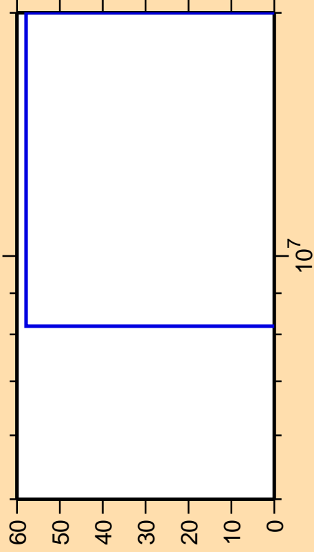
\Delta\sigma/\sigma vs. E for ^{99}\text{In}(n,n\alpha)
