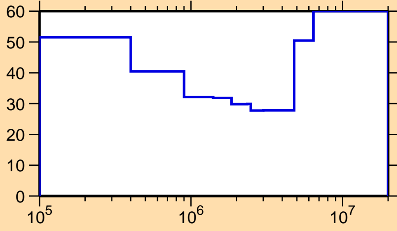
\Delta\sigma/\sigma vs. E for ^{99}\text{In}(n,n_1)
