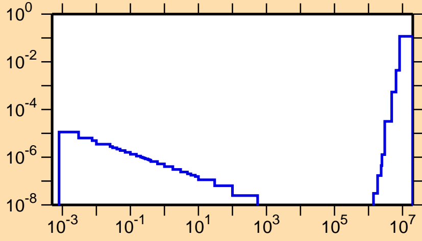
\sigma vs. E for ^{99}\text{In}(n,p)\alpha
