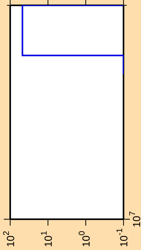
\Delta\sigma/\sigma vs. E for ^{101}\text{In}(n,nt)
