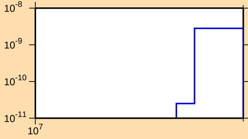
\sigma vs. E for ^{101}\text{In}(\text{mt } 34)
