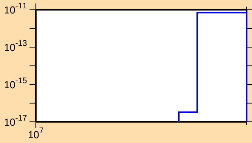
\sigma vs. E for ^{101}\text{In}(n,nt)
