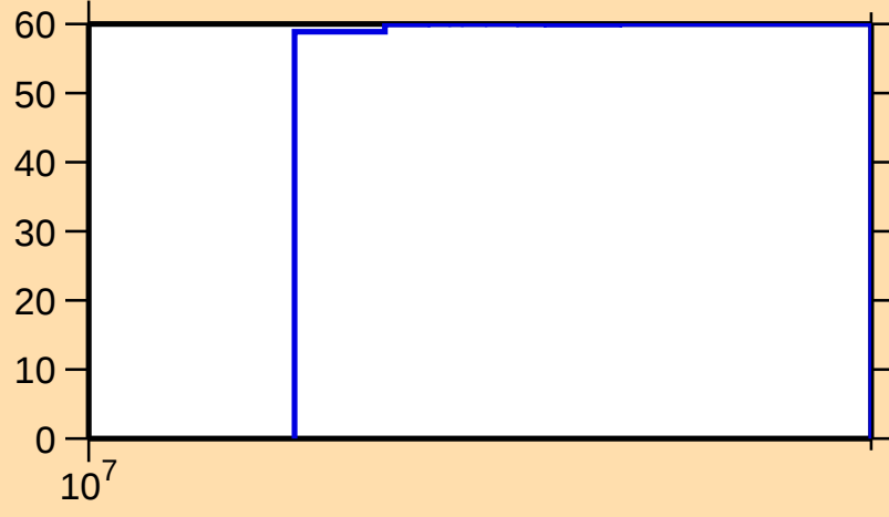
\Delta\sigma/\sigma vs. E for ^{101}\text{In}(n,\text{inel.})
