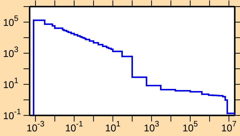
\sigma vs. E for ^{101}\text{In}(n,p)
