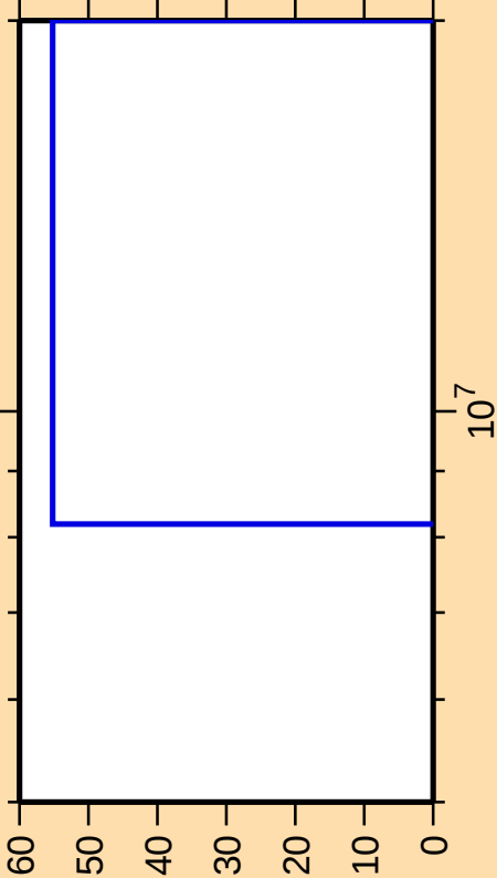
\Delta\sigma/\sigma vs. E for ^{101}\text{In}(n,p)
