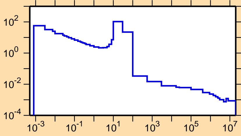
\sigma vs. E for ^{103}\text{In}(n,\gamma)
