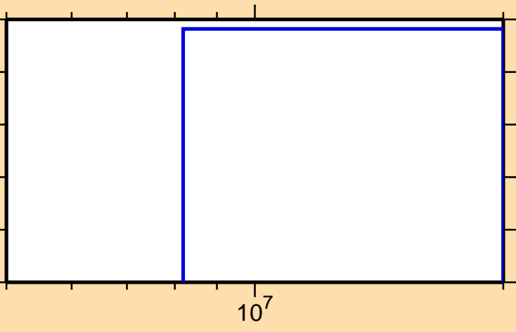
\sigma vs. E for ^{103}\text{In}(n,2n)
