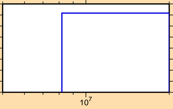
\sigma vs. E for ^{103}\text{In}(\text{mt } 34)
