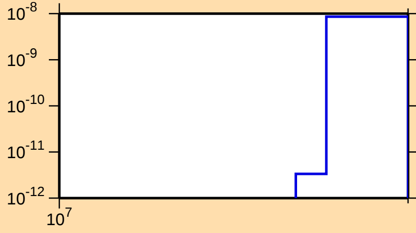
\sigma vs. E for ^{105}\text{In}(n,2n\alpha)
