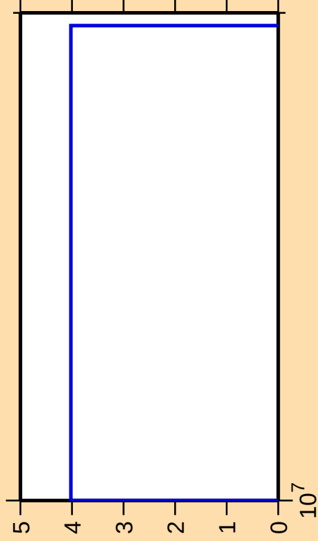
\Delta\sigma/\sigma vs. E for ^{105}\text{In}(\text{mt } 34)
