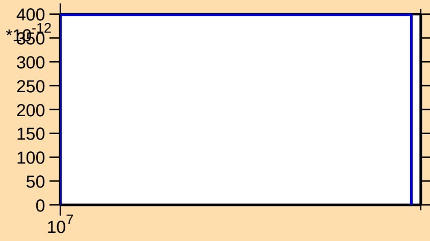
\sigma vs. E for ^{105}\text{In}(n,\text{pt})
