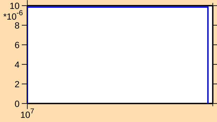
\sigma vs. E for ^{105}\text{In}(n,2np)
