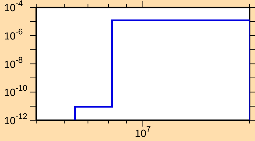
\sigma vs. E for ^{105}\text{In}(n,\text{He3})
