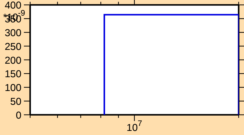
\sigma vs. E for ^{105}\text{In}(n,\text{nd})
