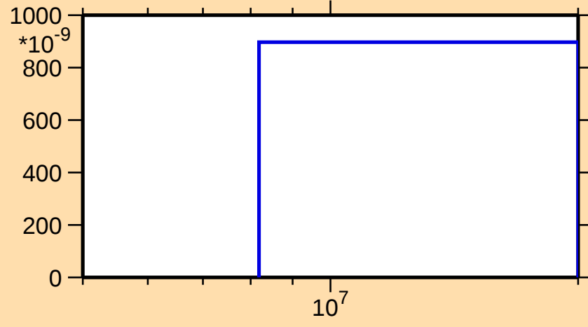
\sigma vs. E for ^{105}\text{In}(\text{mt } 45)
