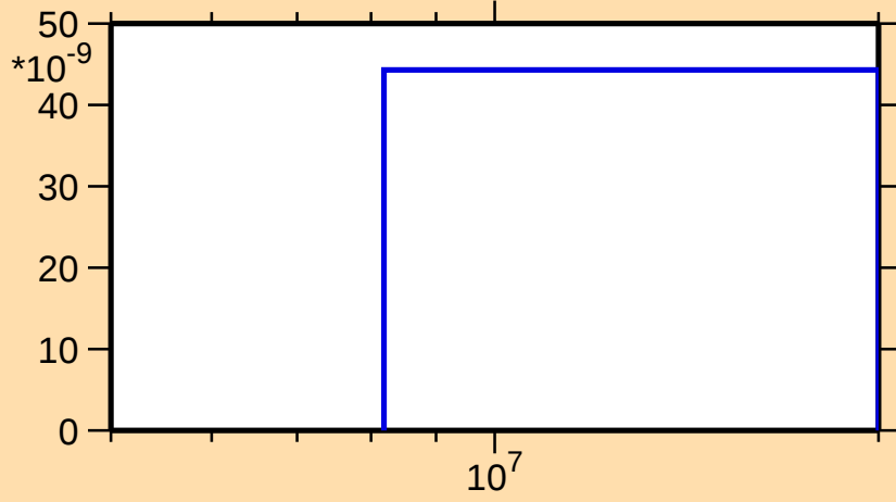
\sigma vs. E for ^{105}\text{In}(\text{mt117})
