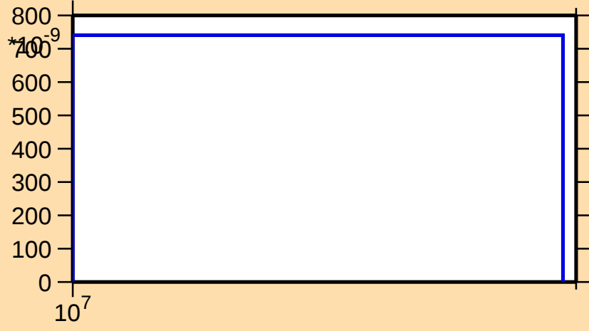
\sigma vs. E for ^{106}\text{In}(\text{mt } 45)
