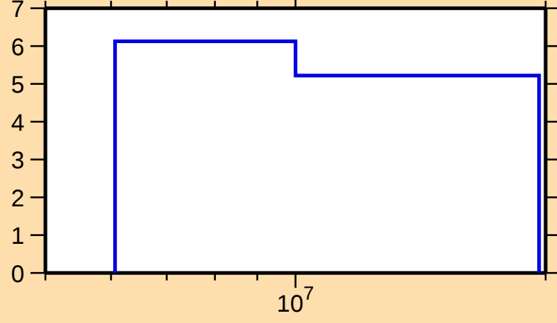
\Delta\sigma/\sigma vs. E for ^{106}\text{In}(n,\text{nonel.})
