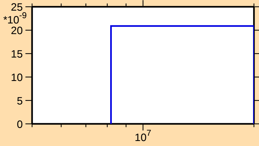
\sigma vs. E for ^{106}\text{In}(\text{mt117})
