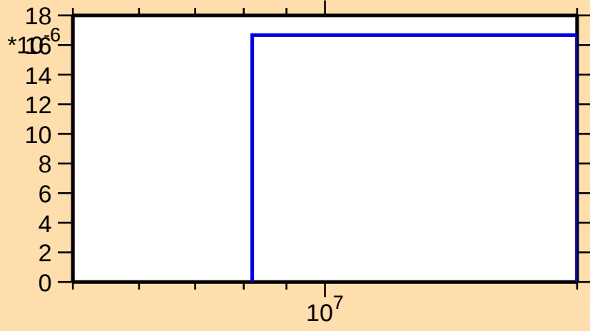
\sigma vs. E for ^{106}\text{In}(n,\text{nd})
