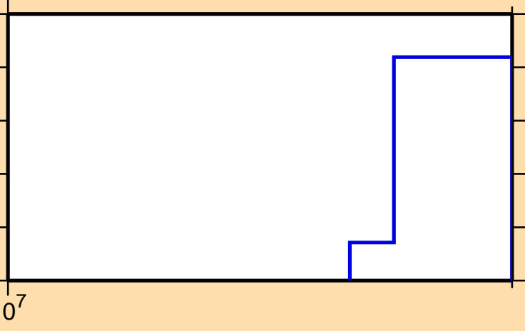
\sigma vs. E for ^{107}\text{In}(n,nt)
