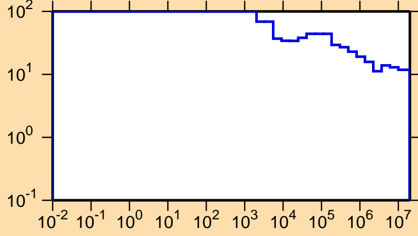
\Delta\sigma/\sigma vs. E for ^{107}\text{In}(n,\text{nonel.})
