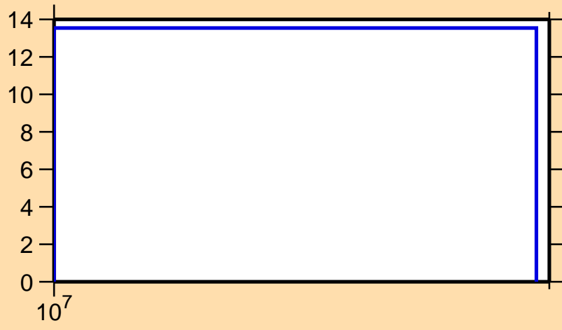
\Delta\sigma/\sigma vs. E for ^{107}\text{In}(n,\text{tot.})
