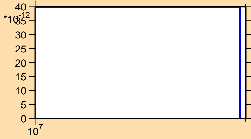
\sigma vs. E for ^{107}\text{In}(n,\text{pt})
