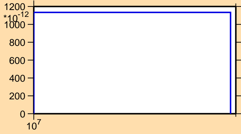
\sigma vs. E for ^{107}\text{In}(n,nt)
