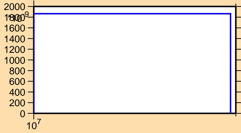
\sigma vs. E for ^{107}\text{In}(n,\text{nd})
