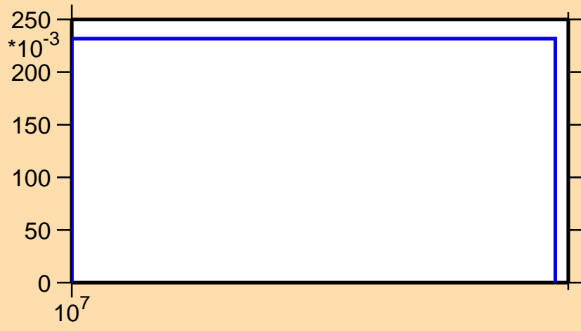
\sigma vs. E for ^{107}\text{In}(n,2n)
