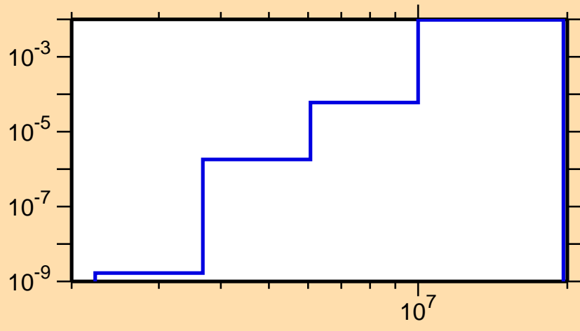
\sigma vs. E for ^{107}\text{In}(n,d)
