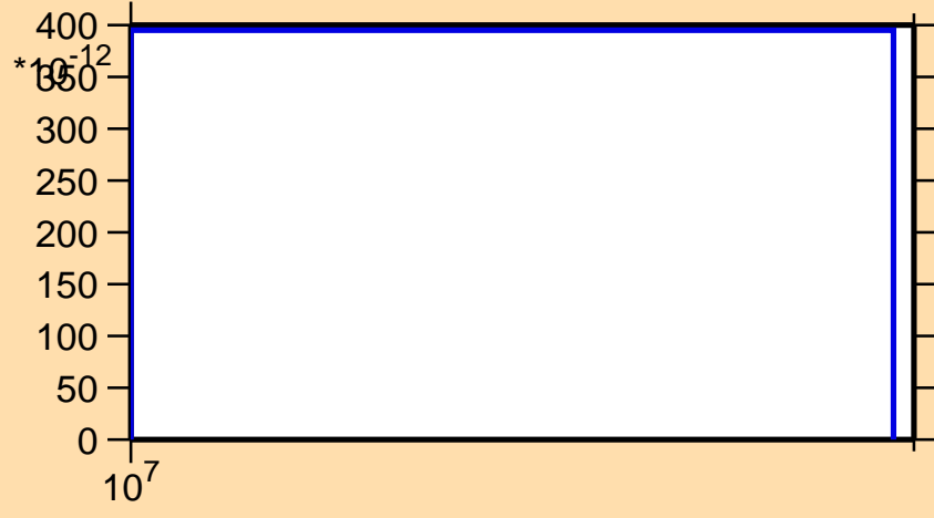
\sigma vs. E for ^{107}\text{In}(n,3n)
