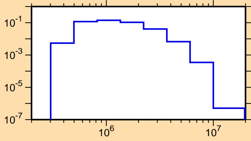
\sigma vs. E for ^{107}\text{In}(n,n_4)
