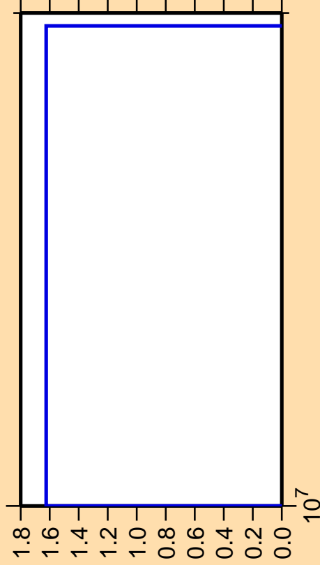
\Delta\sigma/\sigma vs. E for ^{107}\text{In}(\text{mt } 34)
