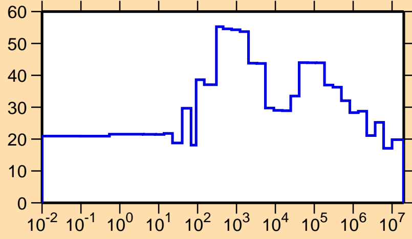
\Delta\sigma/\sigma vs. E for ^{107}\text{In}(n,\text{el.})
