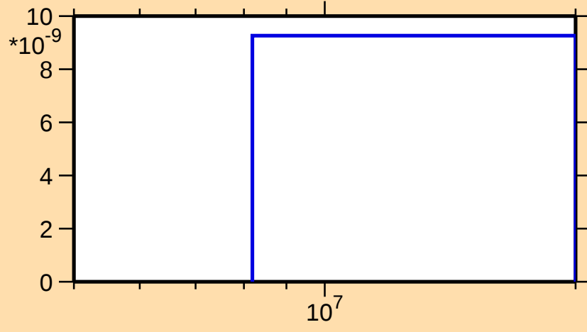
\sigma vs. E for ^{107}\text{In}(n,3n)
