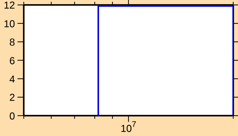
\Delta\sigma/\sigma vs. E for ^{107}\text{In}(n,\text{tot.})
