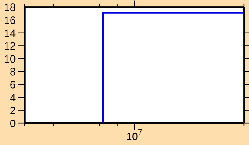
\Delta\sigma/\sigma vs. E for ^{107}\text{In}(n,\text{el.})
