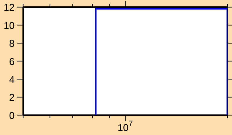
\Delta\sigma/\sigma vs. E for ^{107}\text{In}(n,\text{nonel.})
