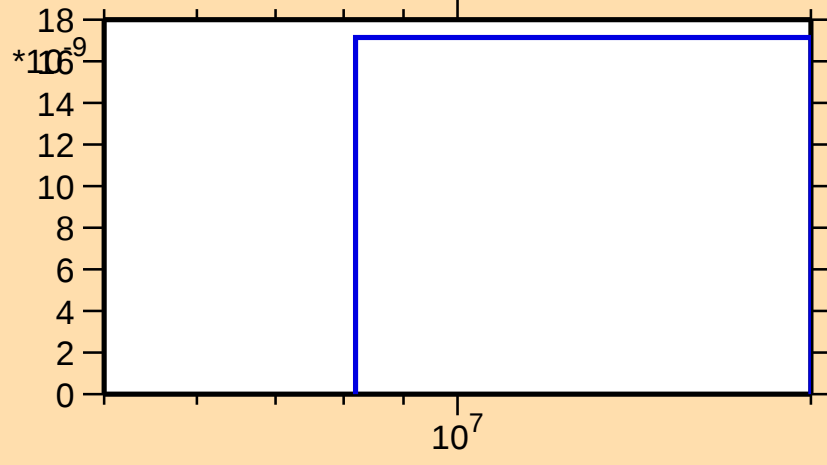
\sigma vs. E for ^{107}\text{In}(\text{mt117})
