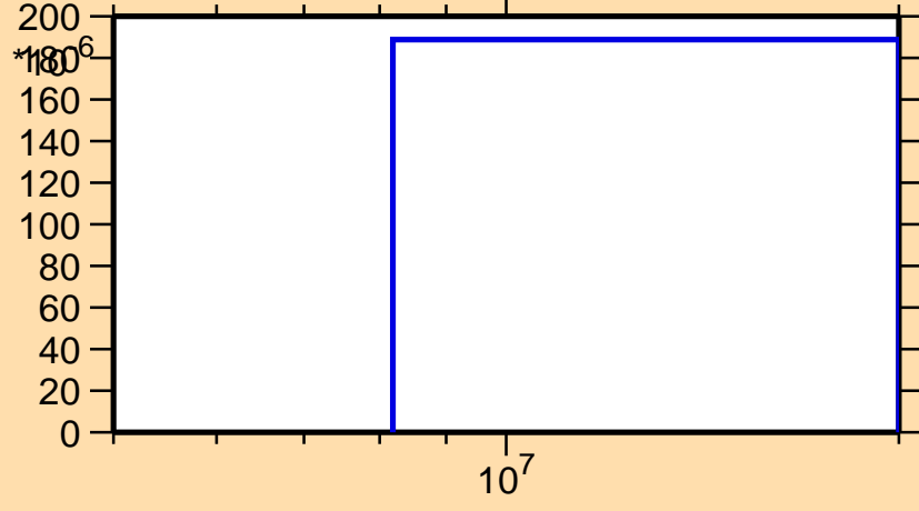
\sigma vs. E for ^{110}\text{In}(n,2np)
