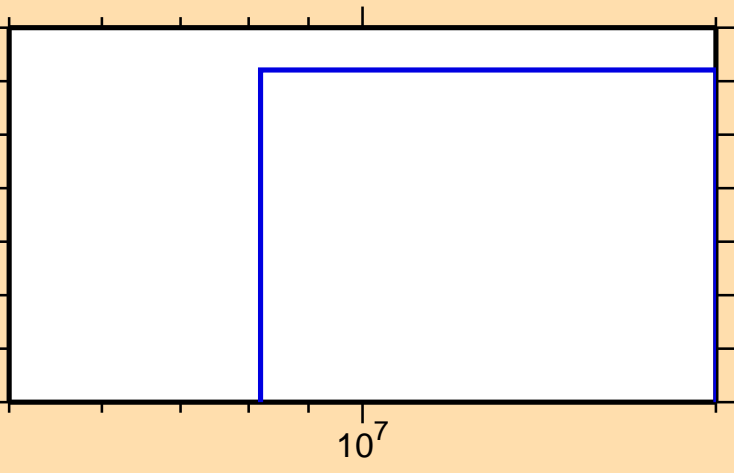
\sigma vs. E for ^{110}\text{In}(n,2n\alpha)
