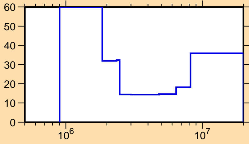
\Delta\sigma/\sigma vs. E for ^{110}\text{In}(n,n\text{cont.})
