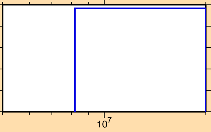
\sigma vs. E for ^{110}\text{In}(n,nd)
