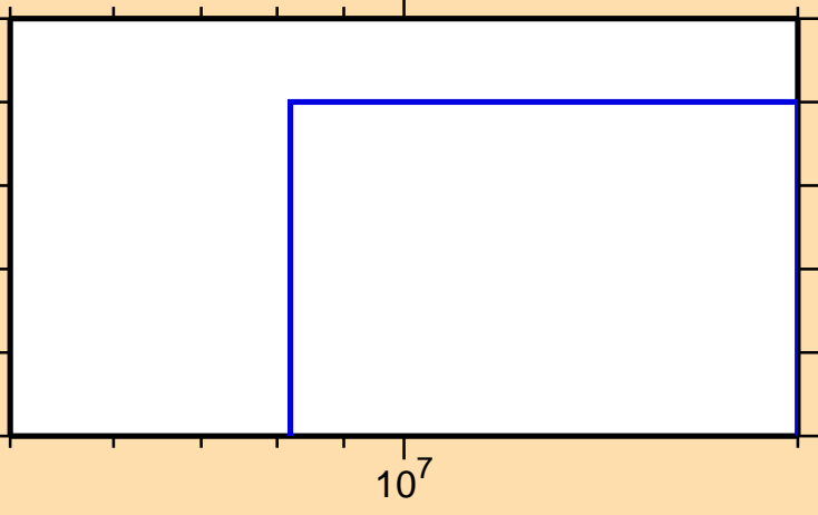
\sigma vs. E for ^{110}\text{In}(n,3n)
