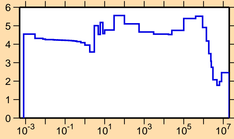
\sigma vs. E for ^{112}\text{In}(n,\text{el.})
