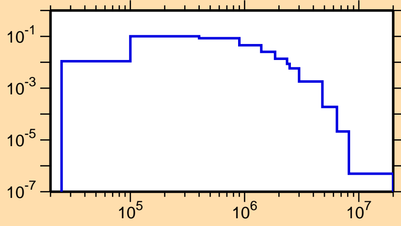
\sigma vs. E for ^{112}\text{In}(n,n_3)
