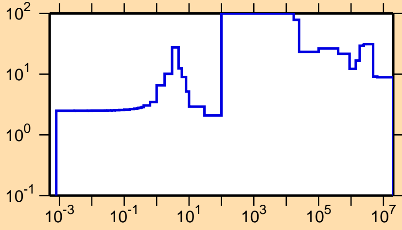
\Delta\sigma/\sigma vs. E for ^{112}\text{In}(n,el.)
