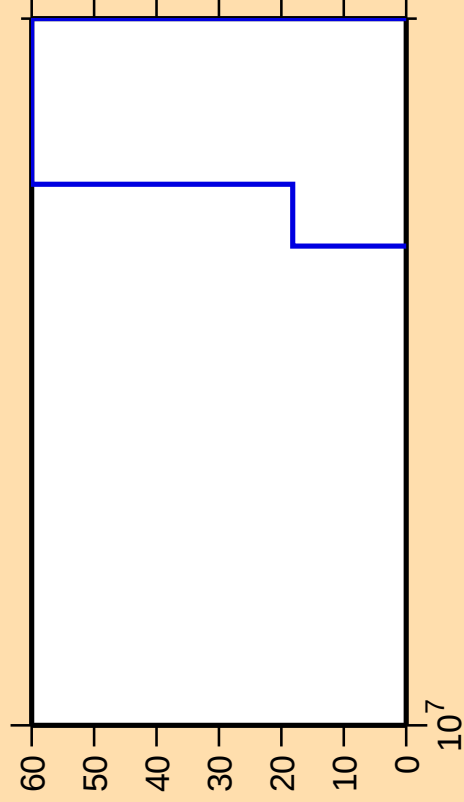
\Delta\sigma/\sigma vs. E for ^{113}\text{In}(n,\text{nt})
