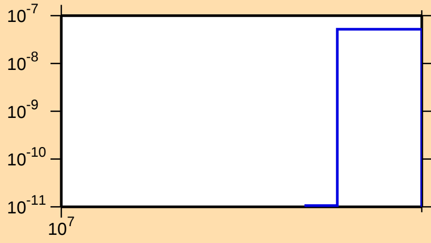
\sigma vs. E for ^{113}\text{In}(n,\text{nt})
