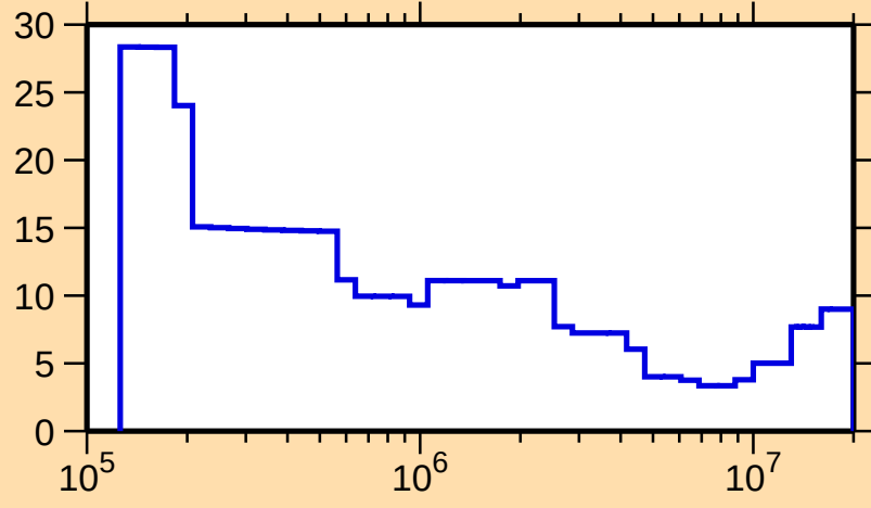
\Delta\sigma/\sigma vs. E for ^{116}\text{In}(n,\text{tot.})
