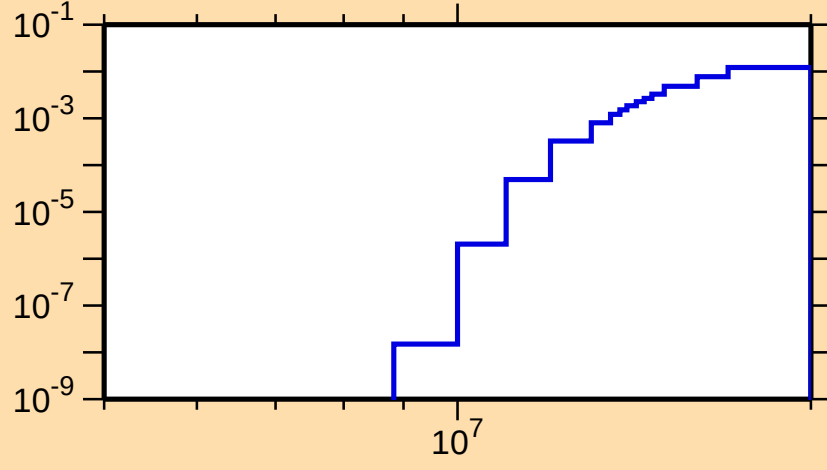
\sigma vs. E for ^{116}\text{In}(n,np)
