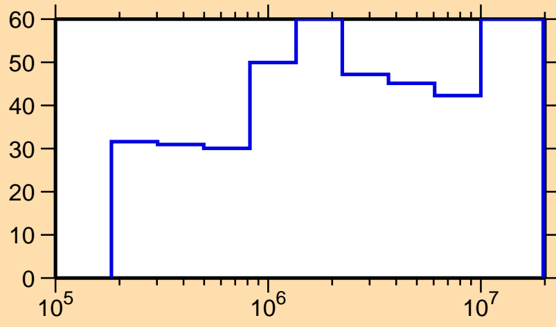
\Delta\sigma/\sigma vs. E for ^{116}\text{In}(n,n_1)
