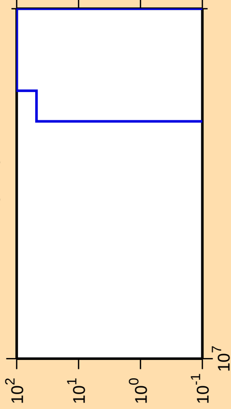
\Delta\sigma/\sigma vs. E for ^{119}\text{In}(n,\text{nt})
