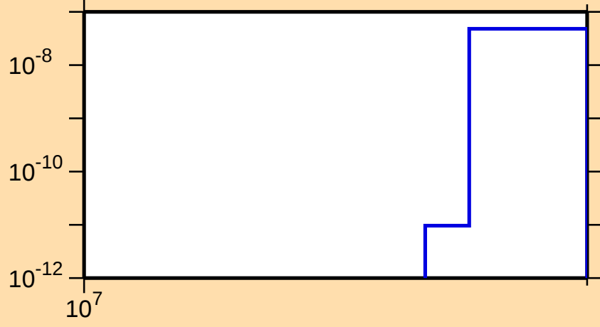
\sigma vs. E for ^{119}\text{In}(n,\text{nt})
