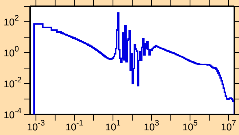
\sigma vs. E for ^{119}\text{In}(n,\gamma)
