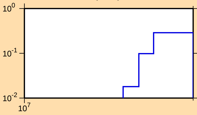
\sigma vs. E for ^{119}\text{In}(n,3n)
