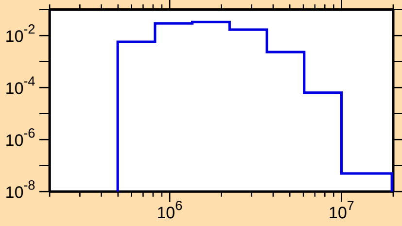
\sigma vs. E for ^{119}\text{In}(n,n_3)
