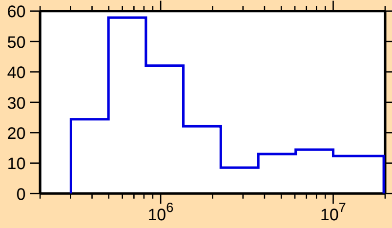
\Delta\sigma/\sigma vs. E for ^{119}\text{In}(\text{n,nonel.})
