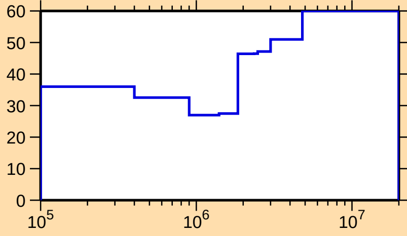
\Delta\sigma/\sigma vs. E for ^{119}\text{In}(n,n_1)
