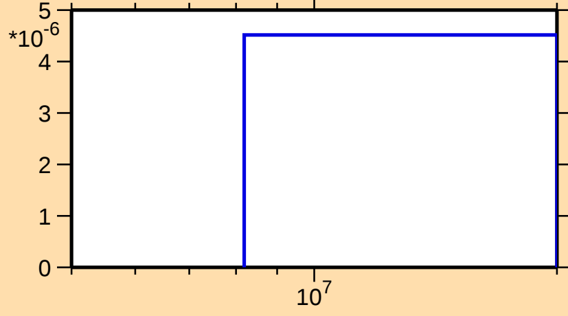
\sigma vs. E for ^{119}\text{In}(n,n\alpha)
