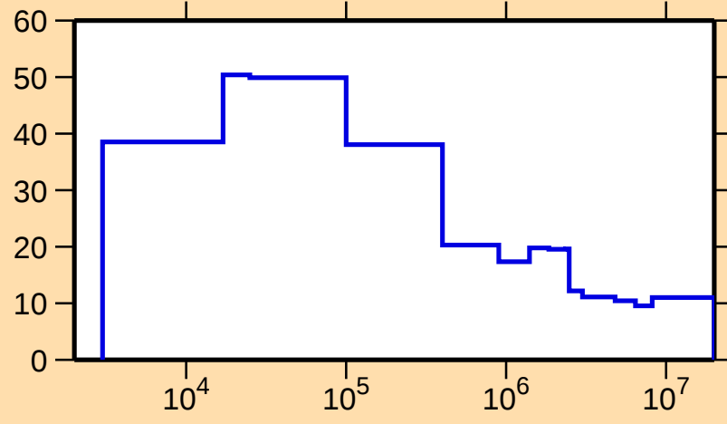
\Delta\sigma/\sigma vs. E for ^{119}\text{In}(n,\text{tot.})
