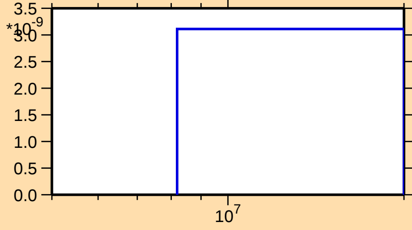
\sigma vs. E for ^{119}\text{In}(n,\text{nd})
