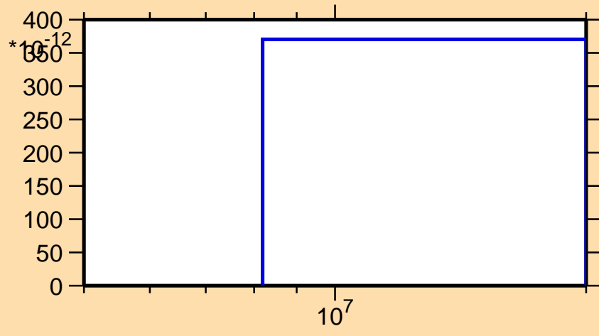
\sigma vs. E for ^{122}\text{In}(n,nt)
