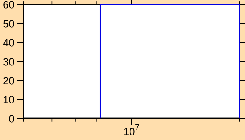
\Delta\sigma/\sigma vs. E for ^{126}\text{In}(\text{n},\text{p})
