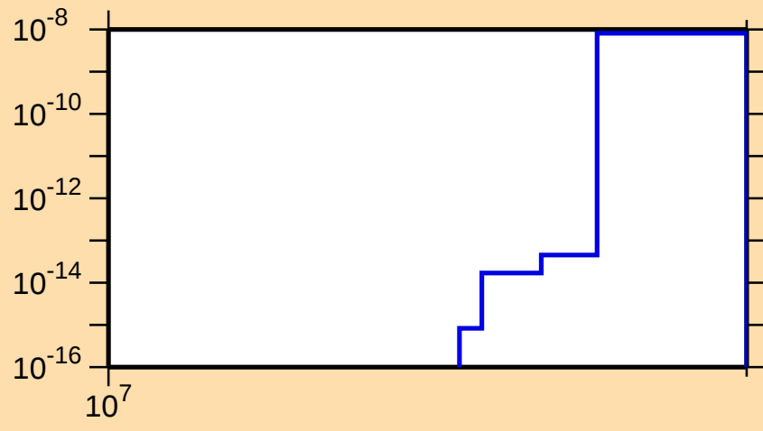
\sigma vs. E for ^{127}\text{In}(n,nt)
