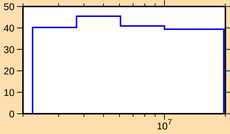
\Delta\sigma/\sigma vs. E for ^{127}\text{In}(n,\text{tot.})
