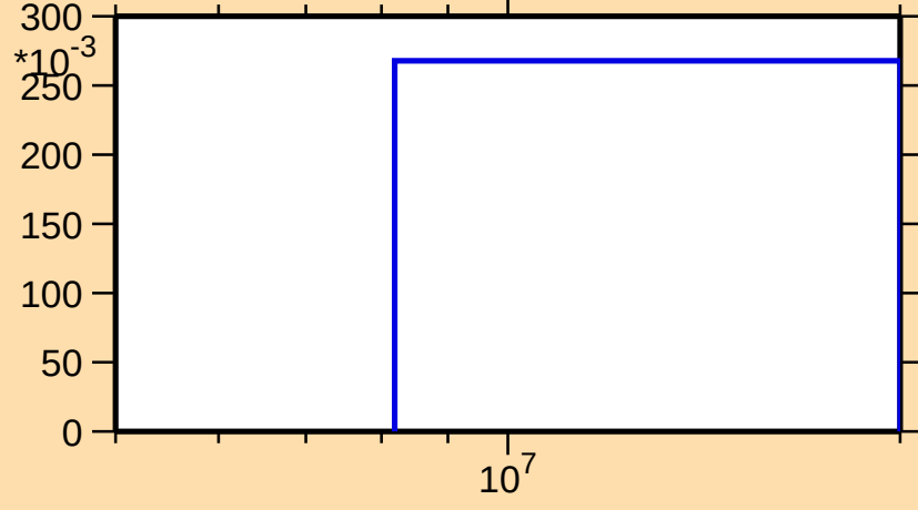
\sigma vs. E for ^{127}\text{In}(n,3n)
