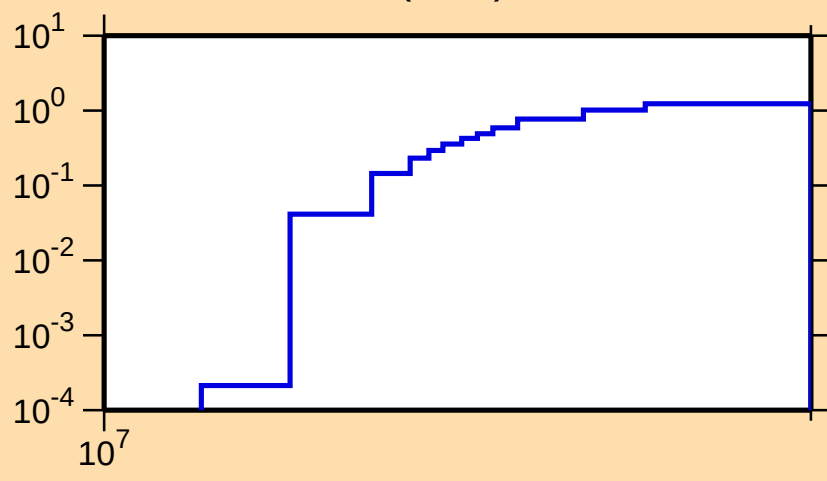
\sigma vs. E for ^{129}\text{In}(n,3n)
