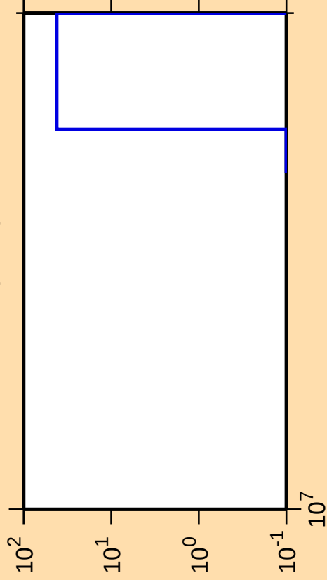
\Delta\sigma/\sigma vs. E for ^{129}\text{In}(n,\text{nd})
