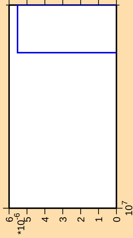
\Delta\sigma/\sigma vs. E for ^{129}\text{In}(n,2np)
