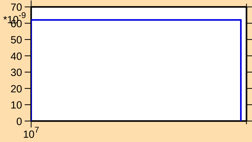
\sigma vs. E for ^{129}\text{In}(n,t)
