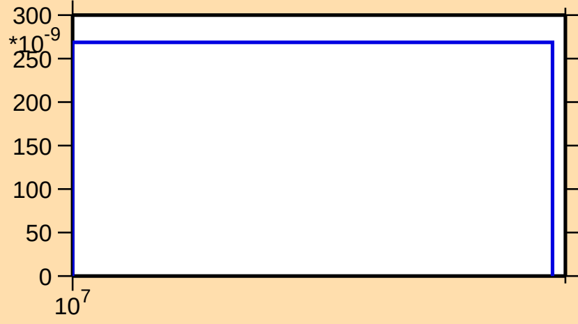
\sigma vs. E for ^{129}\text{In}(n,d)
