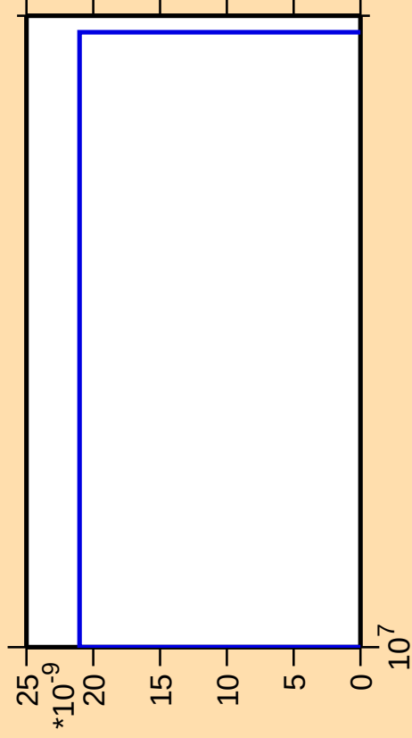
\Delta\sigma/\sigma vs. E for ^{129}\text{In}(n,2np)
