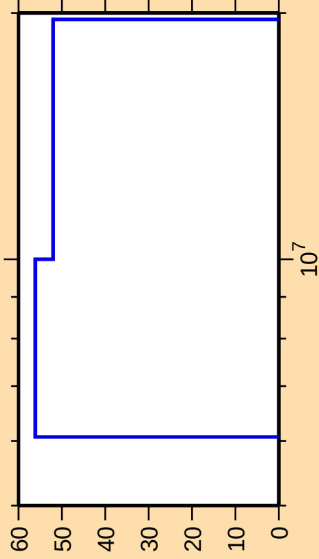
\Delta\sigma/\sigma vs. E for ^{129}\text{In}(n,2n)
