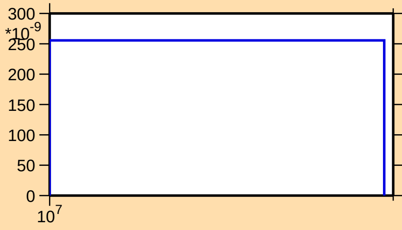
\sigma vs. E for ^{129}\text{In}(n,np)
