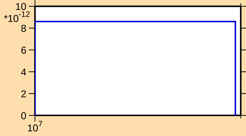
\sigma vs. E for ^{129}\text{In}(n,nt)
