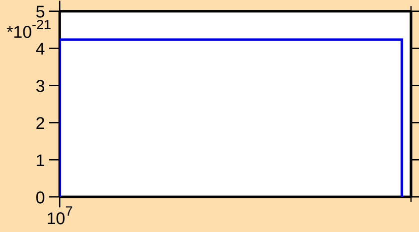
\sigma vs. E for ^{129}\text{In}(n,2np)
