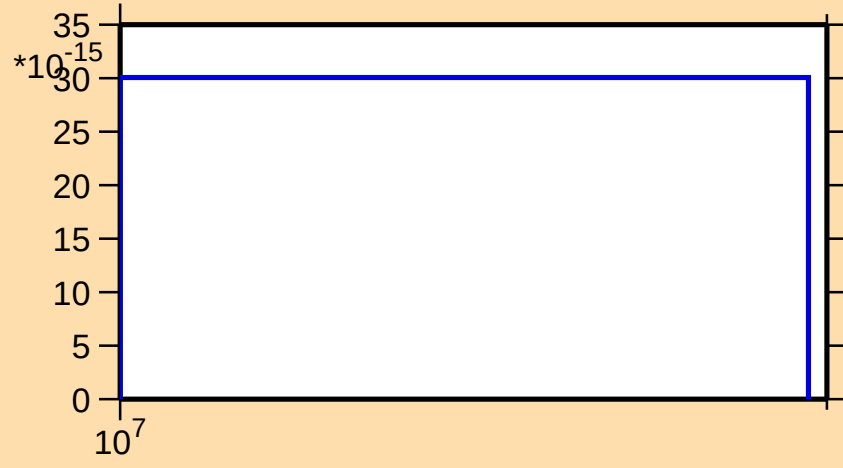
\sigma vs. E for ^{129}\text{In}(n,\text{nd})
