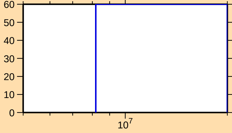
\Delta\sigma/\sigma vs. E for ^{129}\text{In}(n,p)
