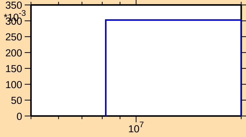
\sigma vs. E for ^{129}\text{In}(n,3n)
