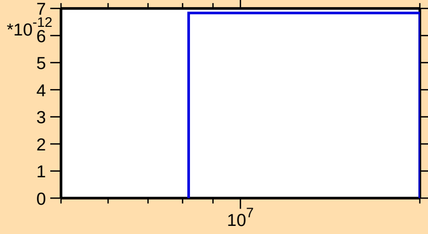
\sigma vs. E for ^{129}\text{In}(n,n\alpha)
