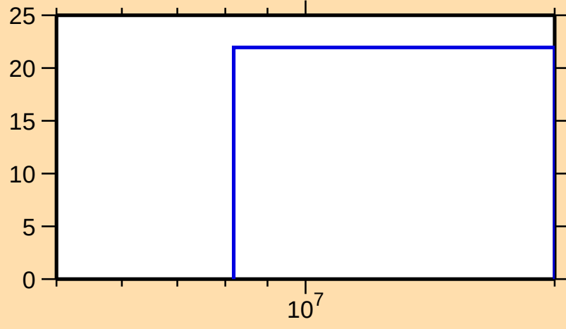
\Delta\sigma/\sigma vs. E for ^{129}\text{In}(n,\text{tot.})
