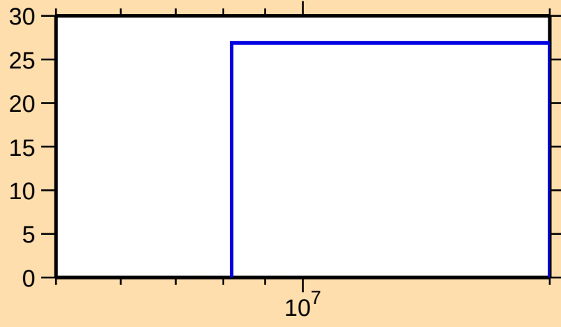
\Delta\sigma/\sigma vs. E for ^{129}\text{In}(n,\text{nonel.})
