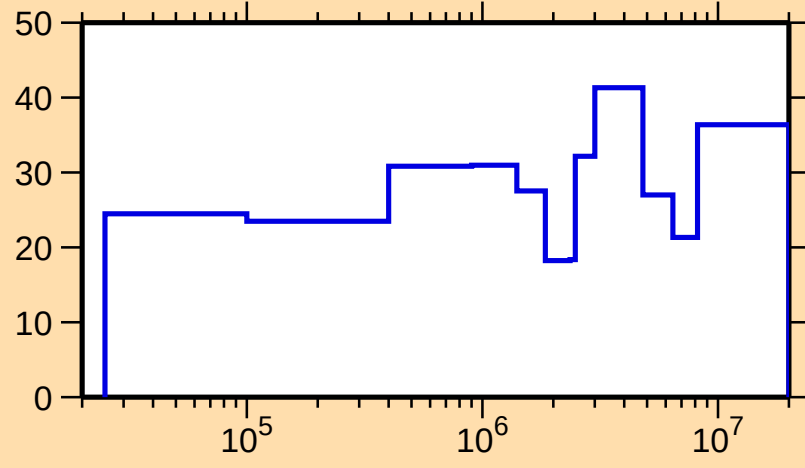
\Delta\sigma/\sigma vs. E for ^{129}\text{In}(n,\text{el.})
