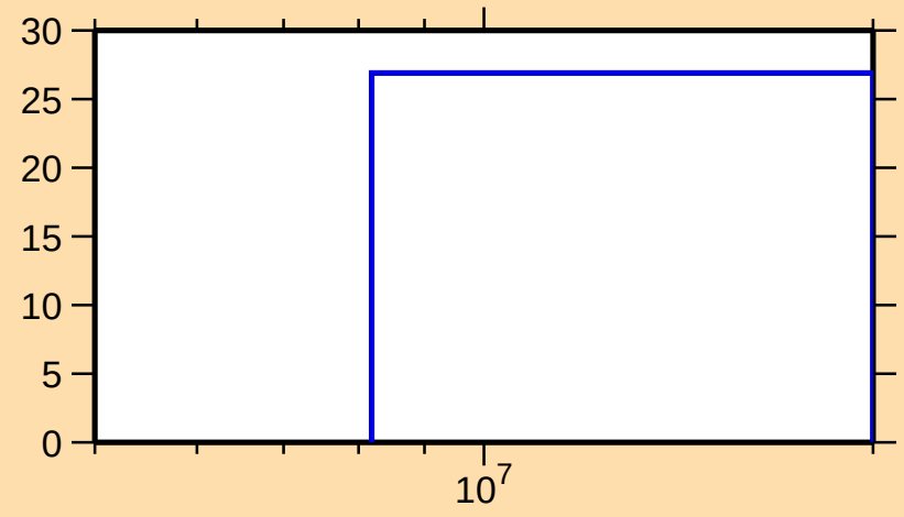
\Delta\sigma/\sigma vs. E for ^{129}\text{In}(n,\text{nonel.})
