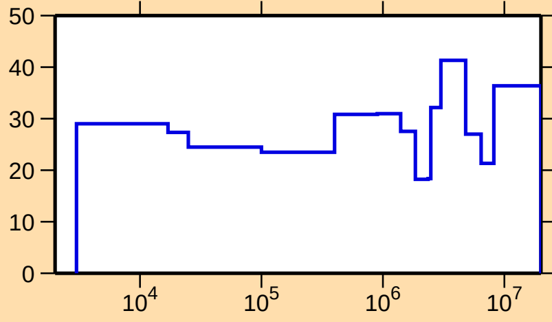
\Delta\sigma/\sigma vs. E for ^{129}\text{In}(n,\text{el.})
