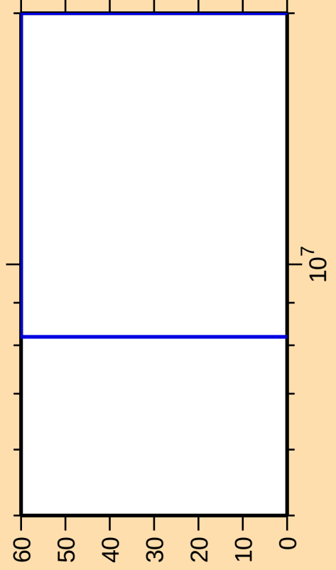
\Delta\sigma/\sigma vs. E for ^{129}\text{In}(n,p)
