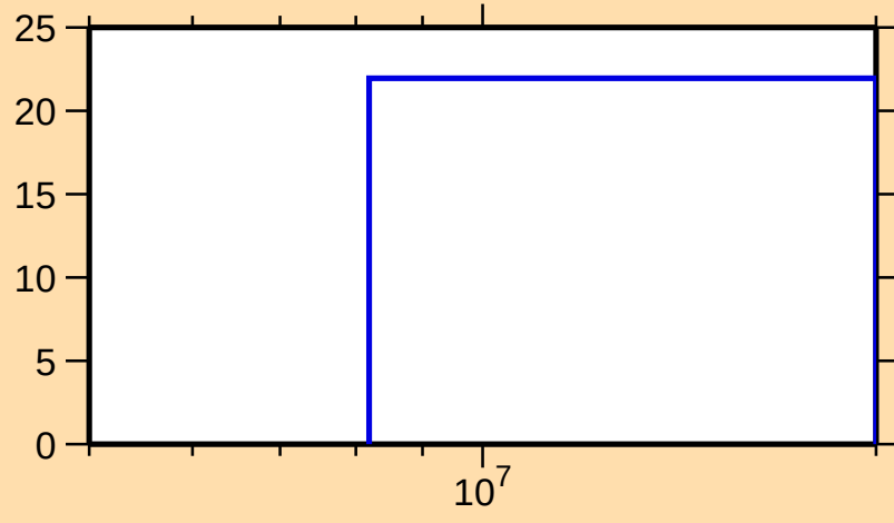
\Delta\sigma/\sigma vs. E for ^{129}\text{In}(n,\text{tot.})
