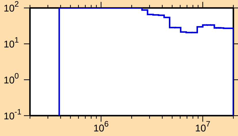
\Delta\sigma/\sigma vs. E for ^{174}\text{Ir}(n,n\text{cont.})
