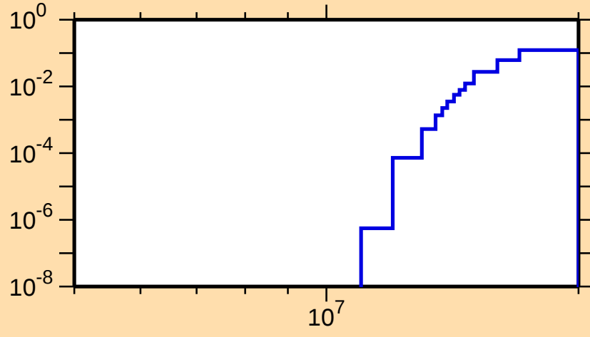
\sigma vs. E for ^{174}\text{Ir}(n,2np)
