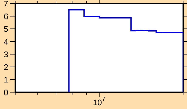
\Delta\sigma/\sigma vs. E for ^{174}\text{Ir}(n,\text{nonel.})
