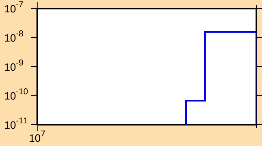
\sigma vs. E for ^{174}\text{Ir}(n,\text{nt})
