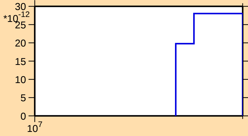
\sigma vs. E for ^{174}\text{Ir}(n,3n\alpha)
