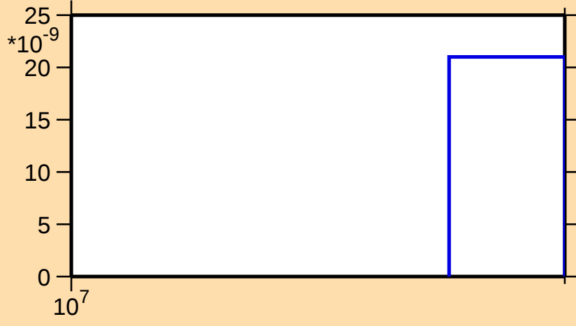
\sigma vs. E for ^{174}\text{Ir}(n,3n)
