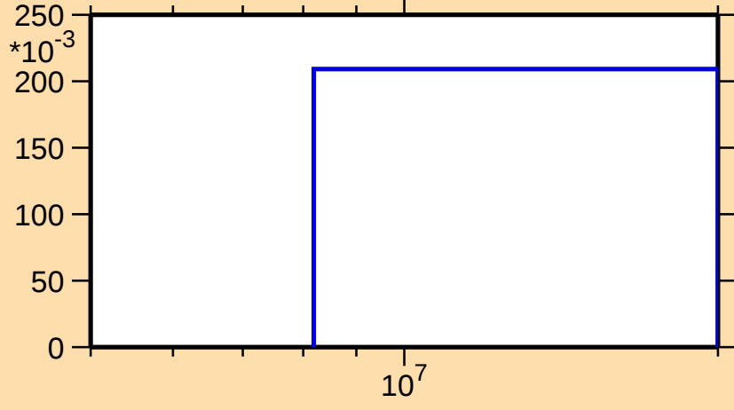
\sigma vs. E for ^{174}\text{Ir}(n,2n)
