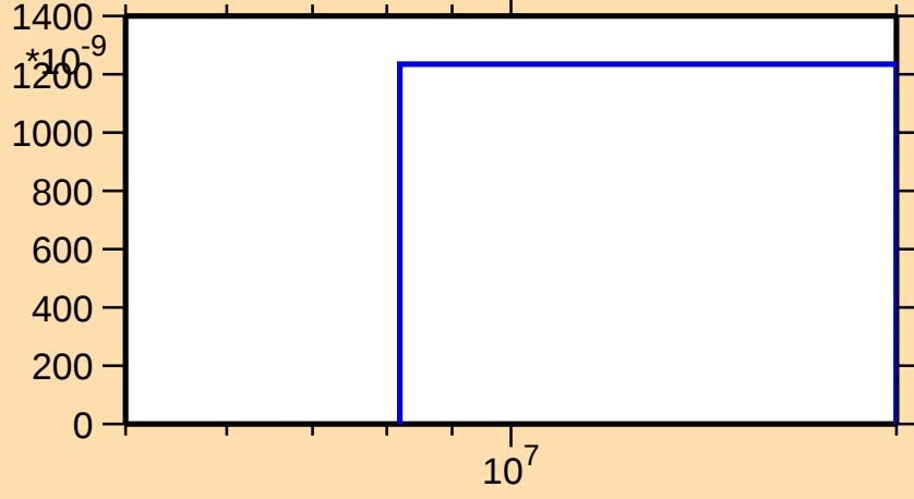
\sigma vs. E for ^{174}\text{Ir}(n,\text{pd})
