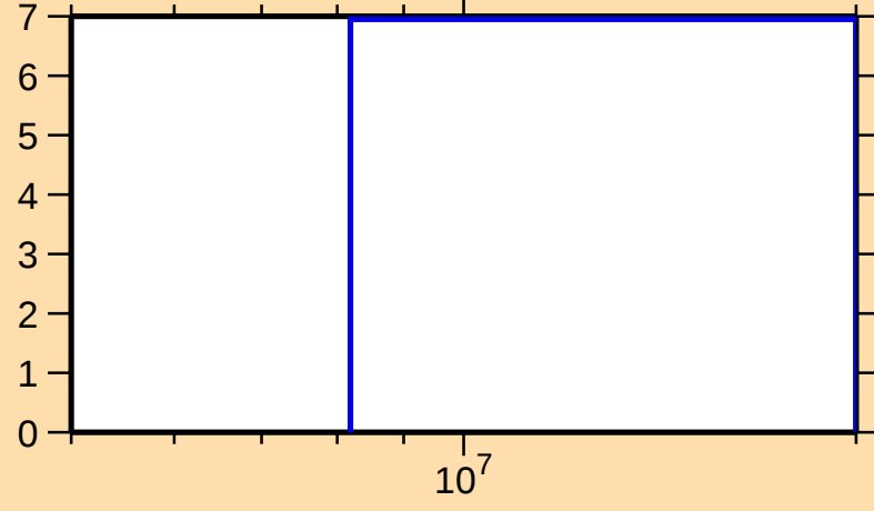
\Delta\sigma/\sigma vs. E for ^{174}\text{Ir}(n,\text{el.})
