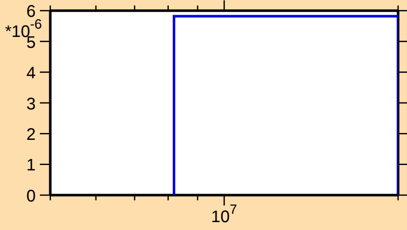
\sigma vs. E for ^{174}\text{Ir}(n,\text{nd})
