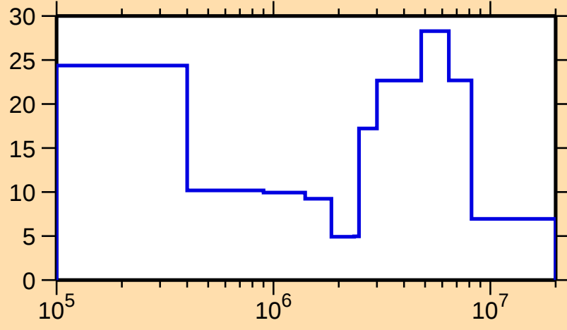
\Delta\sigma/\sigma vs. E for ^{174}\text{Ir}(\text{n,el.})
