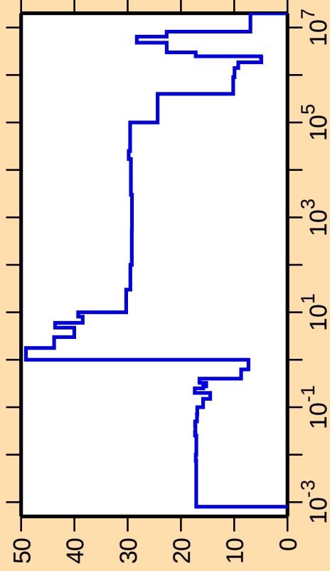
\Delta\sigma/\sigma vs. E for ^{174}\text{Ir}(n,\text{el.})
