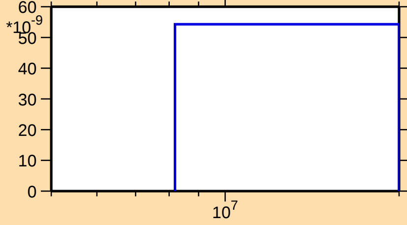
\sigma vs. E for ^{174}\text{Ir}(n,\text{pt})
