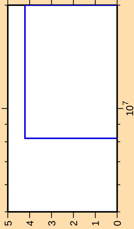
\Delta\sigma/\sigma vs. E for ^{174}\text{Ir}(n,3n\alpha)
