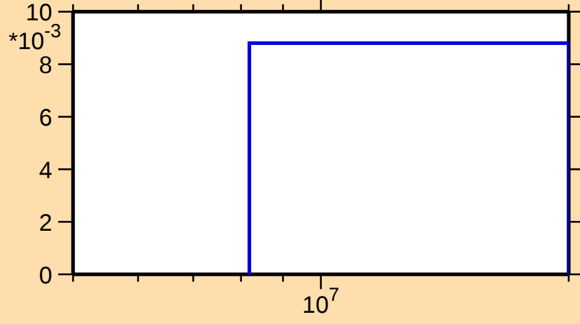
\sigma vs. E for ^{174}\text{Ir}(n,2np)
