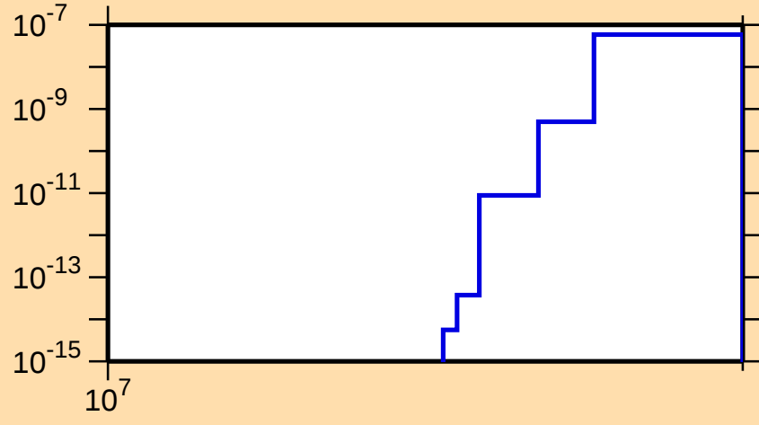
\sigma vs. E for ^{175}\text{Ir}(n,\text{nt})
