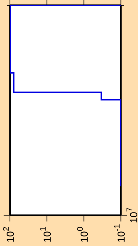
\Delta\sigma/\sigma vs. E for ^{175}\text{Ir}(n,\text{nt})
