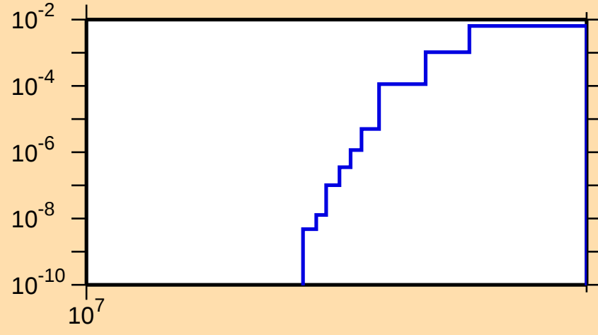
\sigma vs. E for ^{175}\text{Ir}(n,2np)
