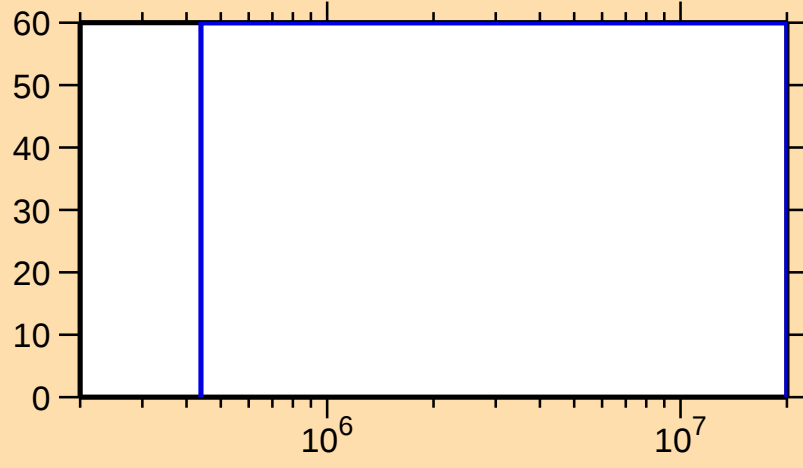
\Delta\sigma/\sigma vs. E for ^{175}\text{Ir}(\text{n},\text{inel.})
