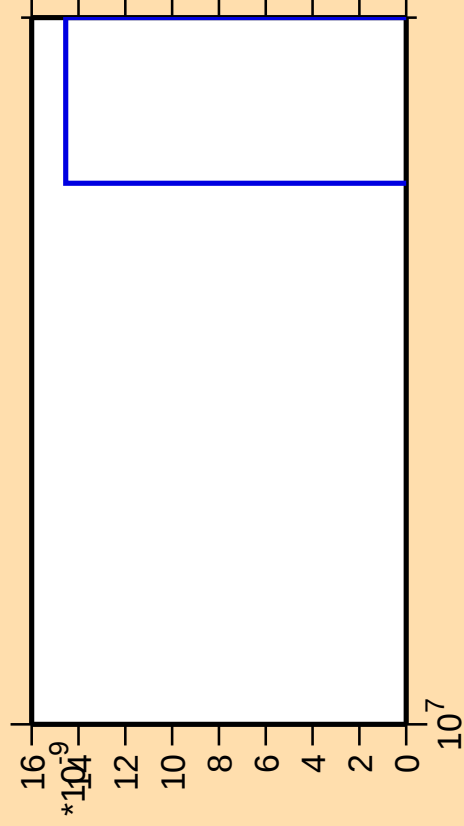
\Delta\sigma/\sigma vs. E for ^{175}\text{Ir}(\text{mt } 42)
