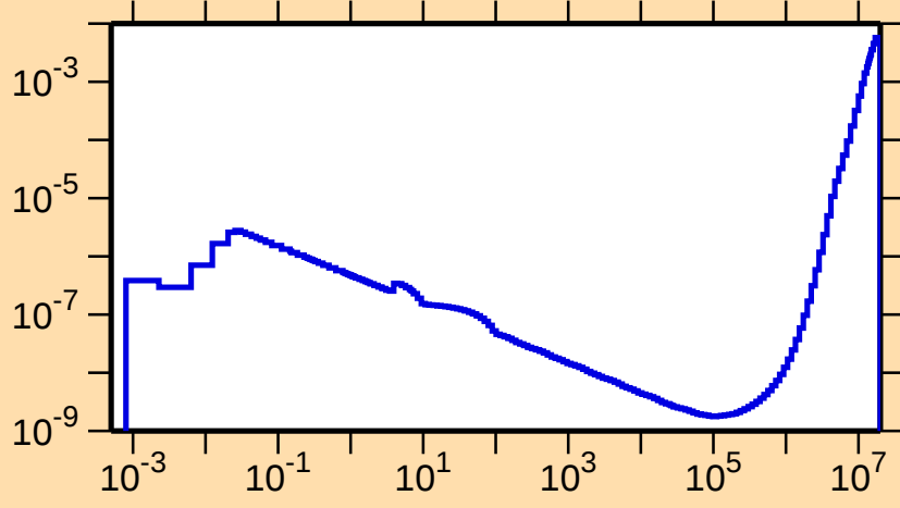
\sigma vs. E for ^{175}\text{Ir}(n,p\alpha)
