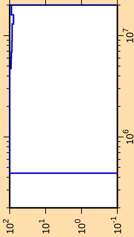
\Delta\sigma/\sigma vs. E for ^{175}\text{Ir}(\text{n},\text{ncont.})
