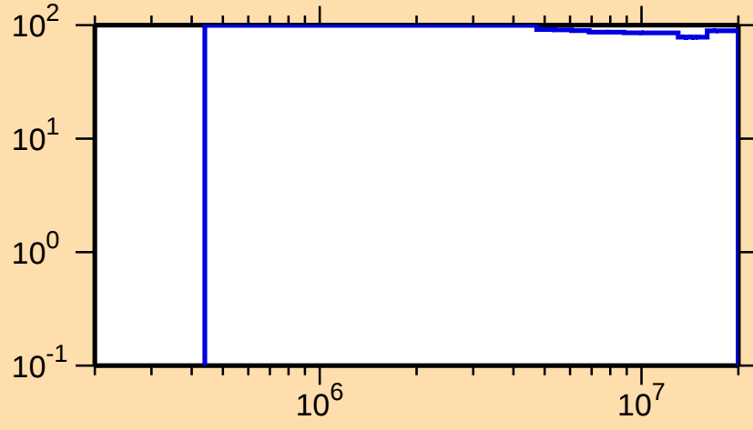
\Delta\sigma/\sigma vs. E for ^{175}\text{Ir}(n,n\text{cont.})
