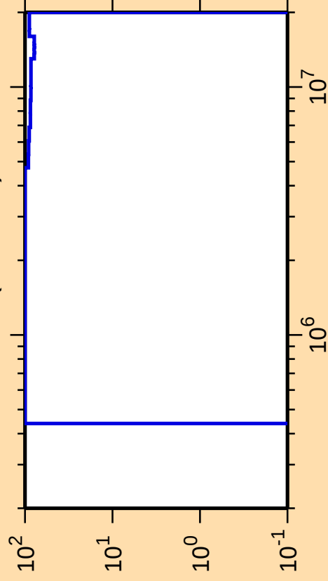
\Delta\sigma/\sigma vs. E for ^{175}\text{Ir}(n,n\text{cont.})
