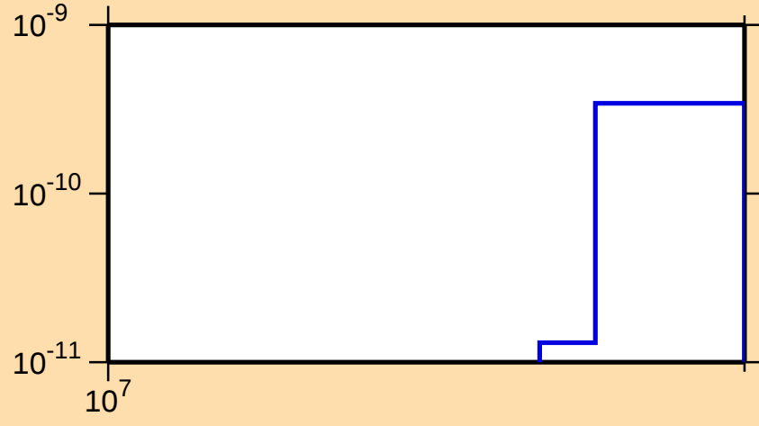
\sigma vs. E for ^{175}\text{Ir}(\text{mt } 34)
