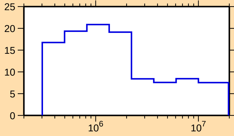
\Delta\sigma/\sigma vs. E for ^{175}\text{Ir}(n,n\text{onel.})
