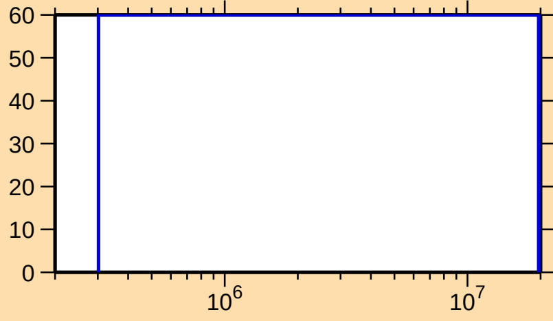
\Delta\sigma/\sigma vs. E for ^{175}\text{Ir}(n,n_1)
