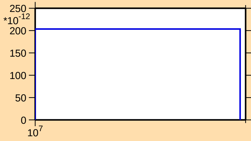
\sigma vs. E for ^{175}\text{Ir}(n,\text{pt})
