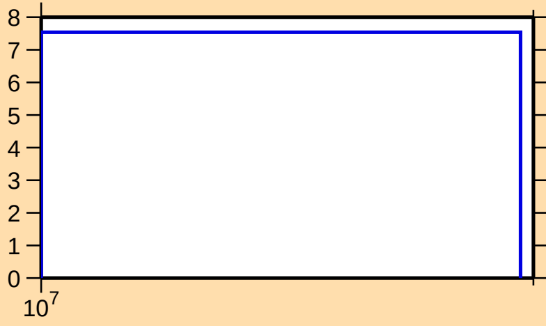
\Delta\sigma/\sigma vs. E for ^{175}\text{Ir}(n,\text{nonel.})
