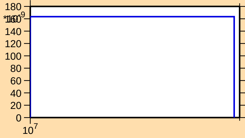
\sigma vs. E for ^{175}\text{Ir}(n,\text{nd})
