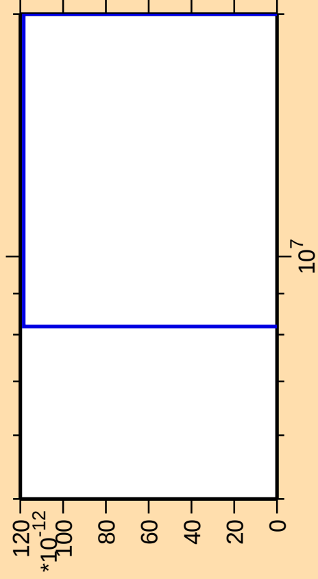
\Delta\sigma/\sigma vs. E for ^{175}\text{Ir}(\text{mt } 42)
