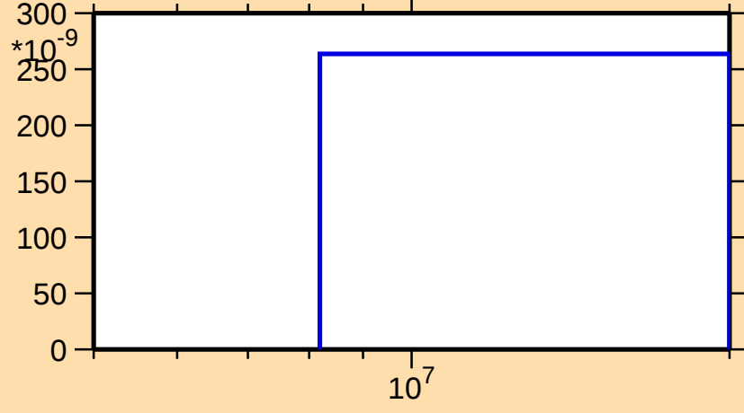
\sigma vs. E for ^{175}\text{Ir}(n,\text{pd})
