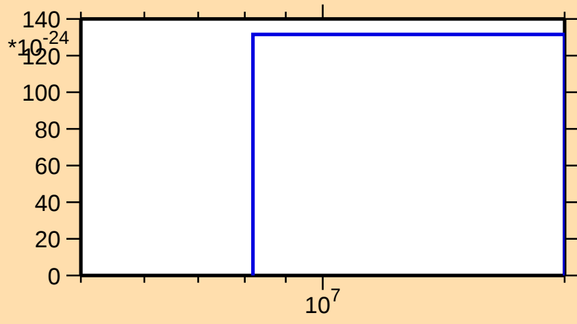
\sigma vs. E for ^{175}\text{Ir}(\text{mt } 42)
