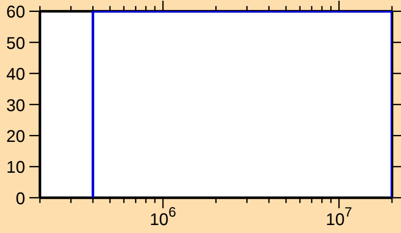
\Delta\sigma/\sigma vs. E for ^{175}\text{Ir}(\text{n},\text{inel.})
