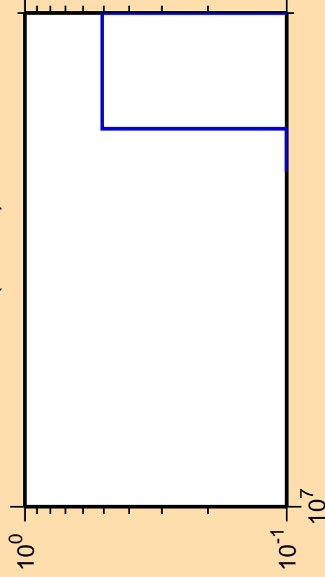
\Delta\sigma/\sigma vs. E for ^{176}\text{Ir}(n,3n\alpha)
