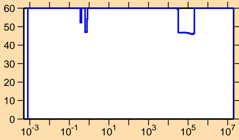
\Delta\sigma/\sigma vs. E for ^{176}\text{Ir}(n,\gamma)
