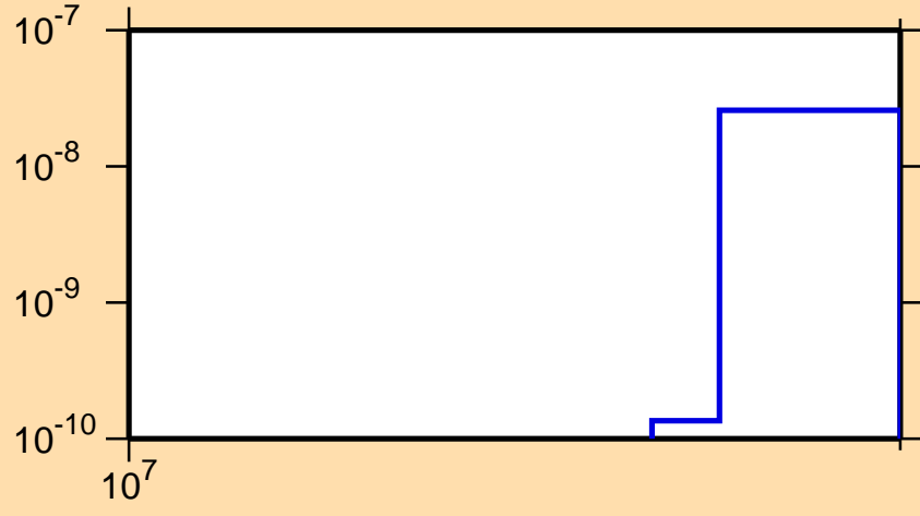
\sigma vs. E for ^{176}\text{Ir}(n,nt)
