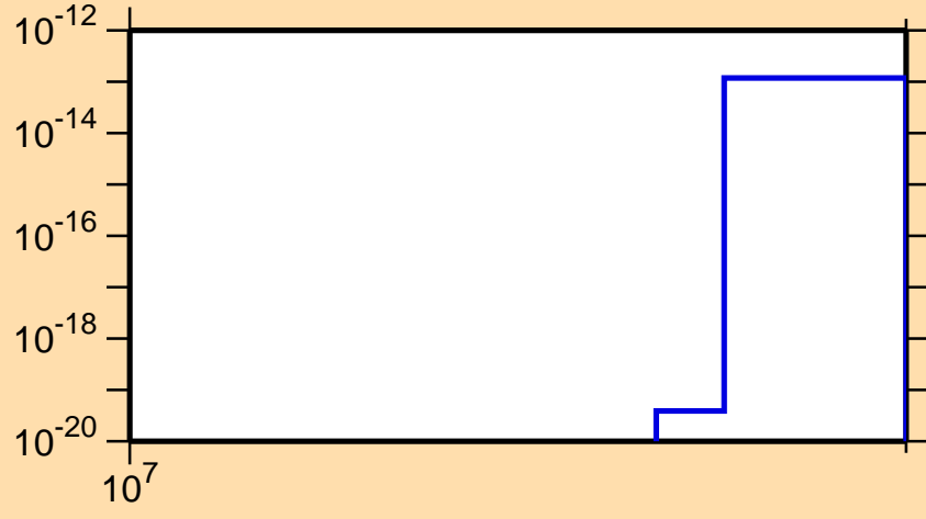
\sigma vs. E for ^{176}\text{Ir}(n,3n\alpha)
