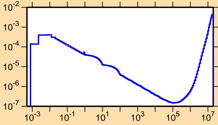
\sigma vs. E for ^{176}\text{Ir}(n,p\alpha)
