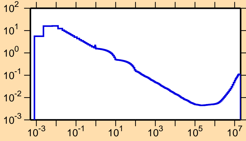
\sigma vs. E for ^{176}\text{Ir}(n,\alpha)
