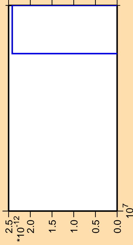
\Delta\sigma/\sigma vs. E for ^{176}\text{Ir}(\text{mt } 42)
