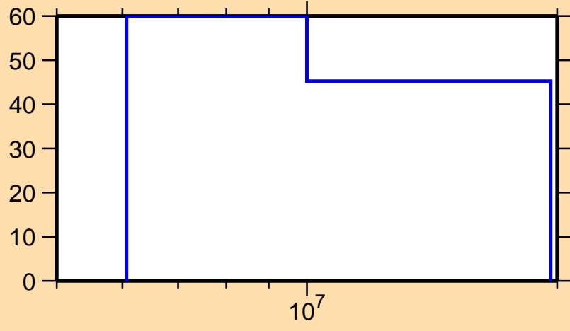
\Delta\sigma/\sigma vs. E for ^{176}\text{Ir}(n,2n)
