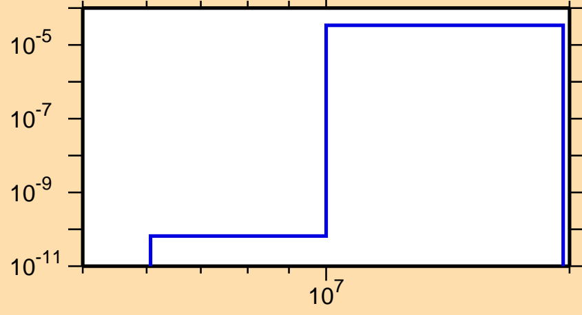
\sigma vs. E for ^{176}\text{Ir}(n,2n\alpha)
