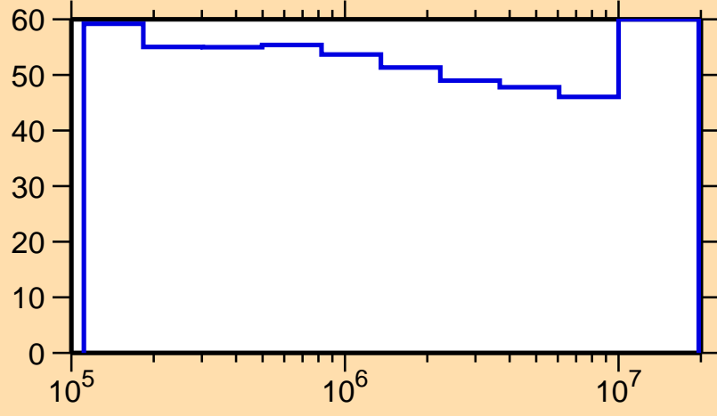
\Delta\sigma/\sigma vs. E for ^{176}\text{Ir}(n,n_1)
