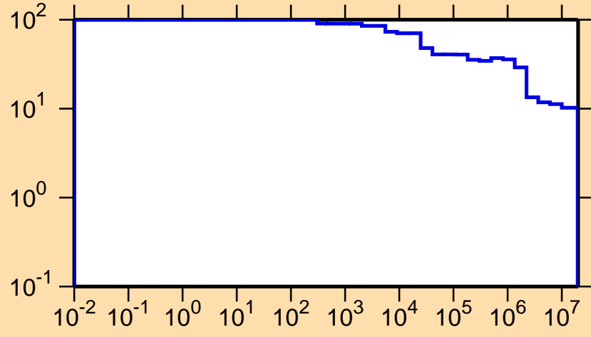
\Delta\sigma/\sigma vs. E for ^{176}\text{Ir}(n,\text{nonel.})
