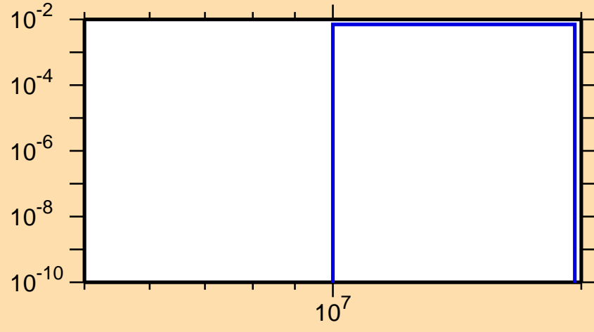
\sigma vs. E for ^{176}\text{Ir}(n,2np)
