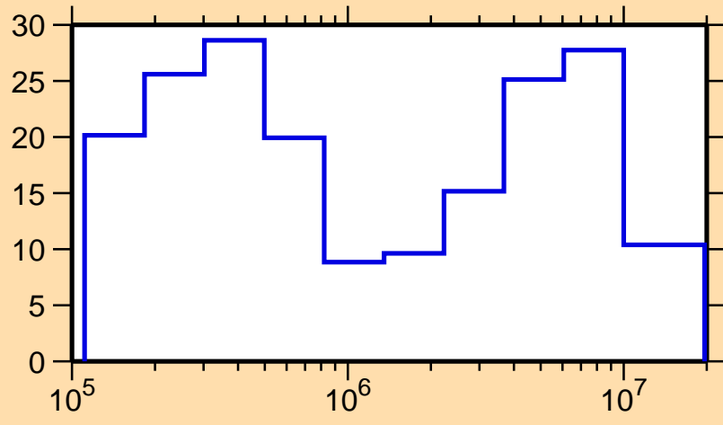
\Delta\sigma/\sigma vs. E for ^{176}\text{Ir}(n,\text{el.})
