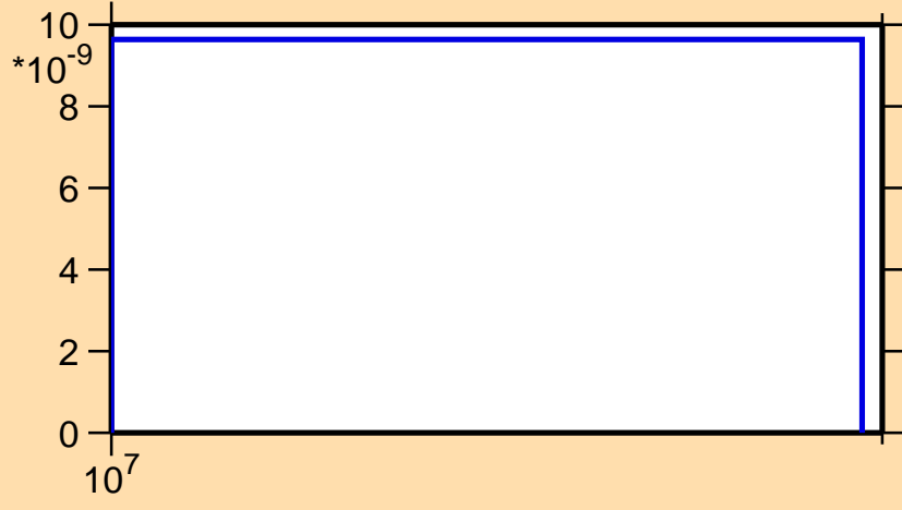
\sigma vs. E for ^{176}\text{Ir}(n,3n)
