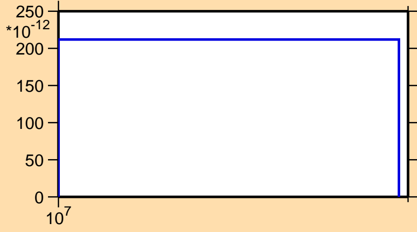
\sigma vs. E for ^{176}\text{Ir}(n,nt)
