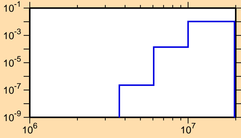
\sigma vs. E for ^{176}\text{Ir}(n,d)
