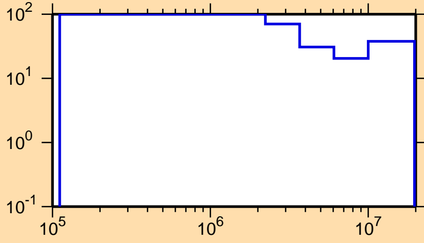
\Delta\sigma/\sigma vs. E for ^{176}\text{Ir}(n,\text{inel.})
