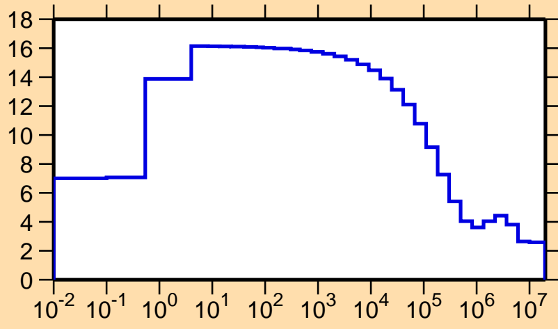
\sigma vs. E for ^{176}\text{Ir}(n,\text{el.})
