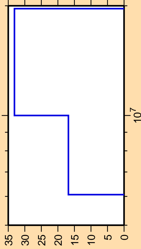
\Delta\sigma/\sigma vs. E for ^{176}\text{Ir}(n,n\text{cont.})
