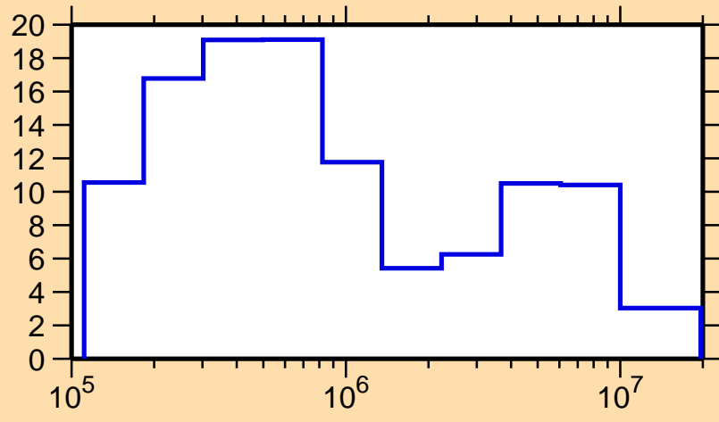
\Delta\sigma/\sigma vs. E for ^{176}\text{Ir}(n,\text{tot.})
