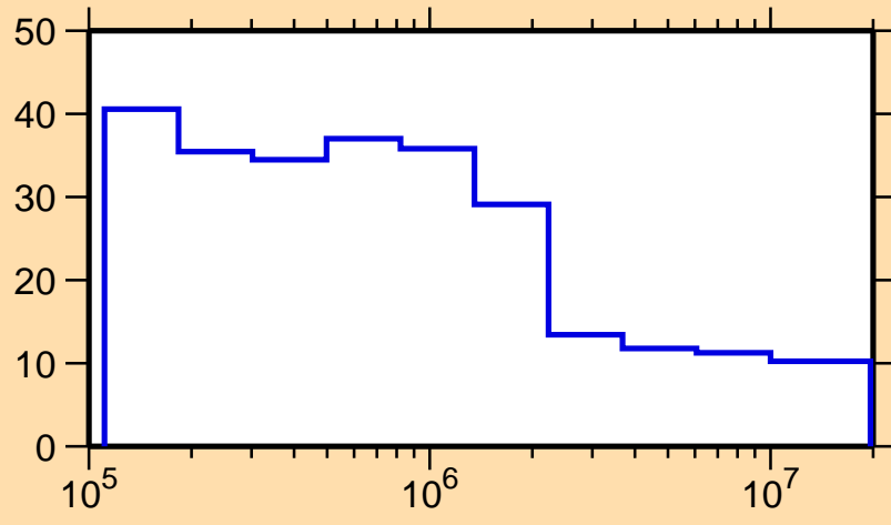
\Delta\sigma/\sigma vs. E for ^{176}\text{Ir}(n,\text{nonel.})
