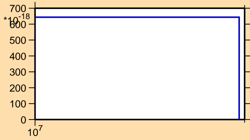
\sigma vs. E for ^{176}\text{Ir}(n,3n\alpha)
