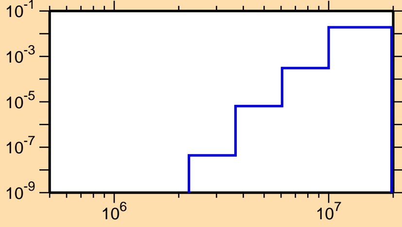
\sigma vs. E for ^{176}\text{Ir}(n,n\alpha)
