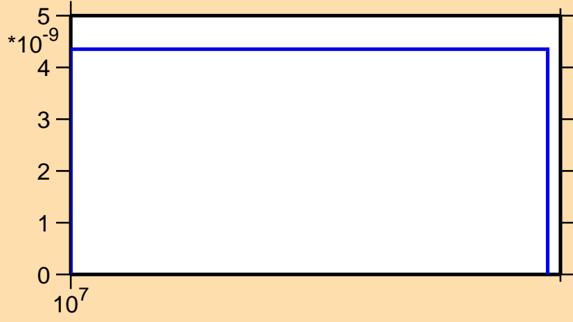
\sigma vs. E for ^{176}\text{Ir}(n,\text{pt})
