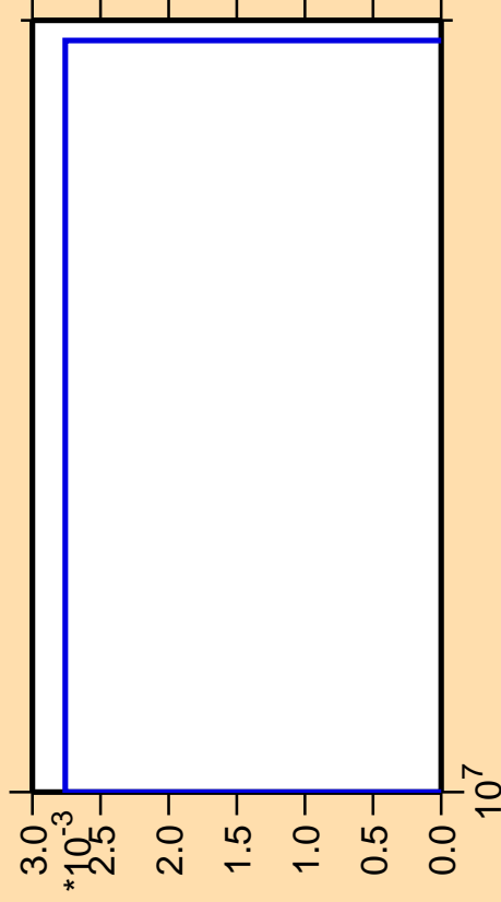
\Delta\sigma/\sigma vs. E for ^{176}\text{Ir}(n,3n\alpha)
