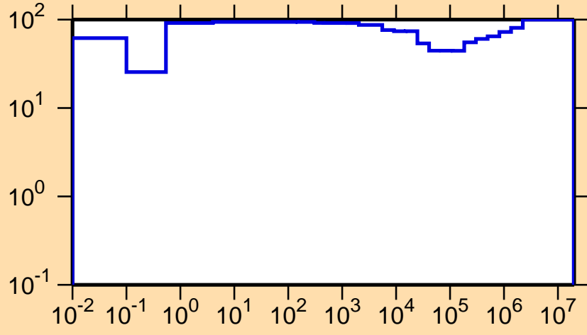
\Delta\sigma/\sigma vs. E for ^{176}\text{Ir}(n,\gamma)
