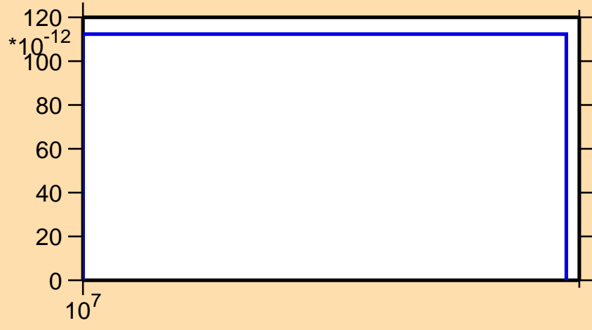
\sigma vs. E for ^{176}\text{Ir}(\text{mt } 34)
