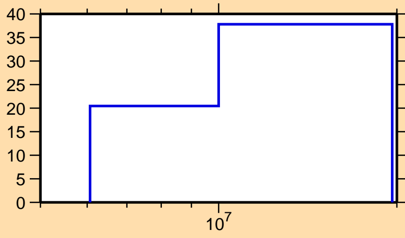
\Delta\sigma/\sigma vs. E for ^{176}\text{Ir}(n,\text{inel.})
