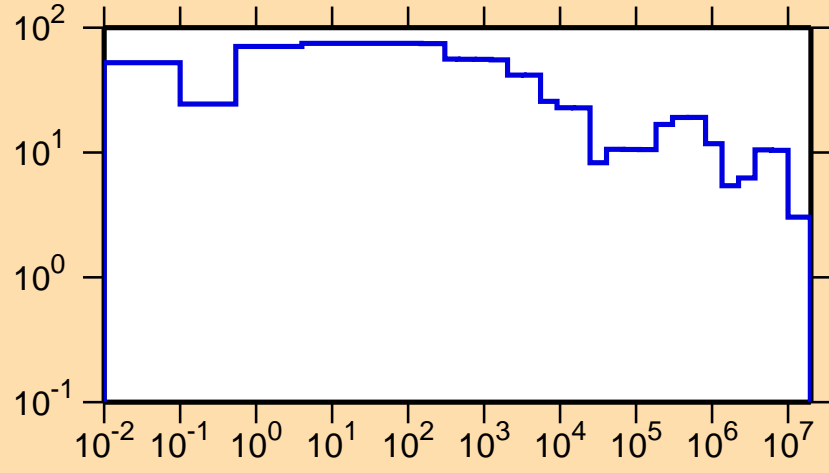
\Delta\sigma/\sigma vs. E for ^{176}\text{Ir}(n,\text{tot.})
