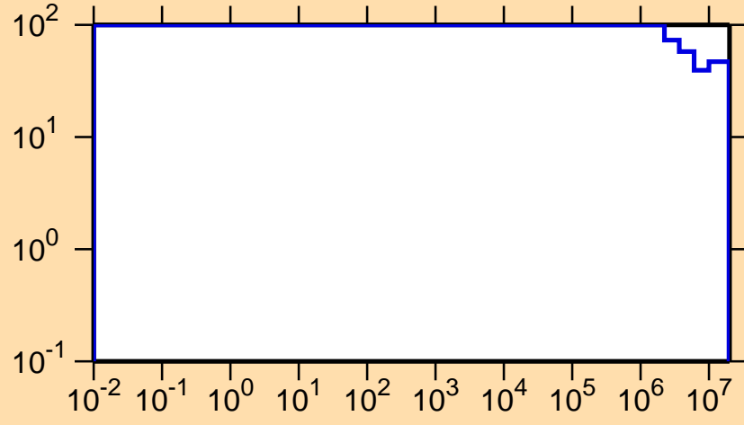
\Delta\sigma/\sigma vs. E for ^{176}\text{Ir}(n,p)
