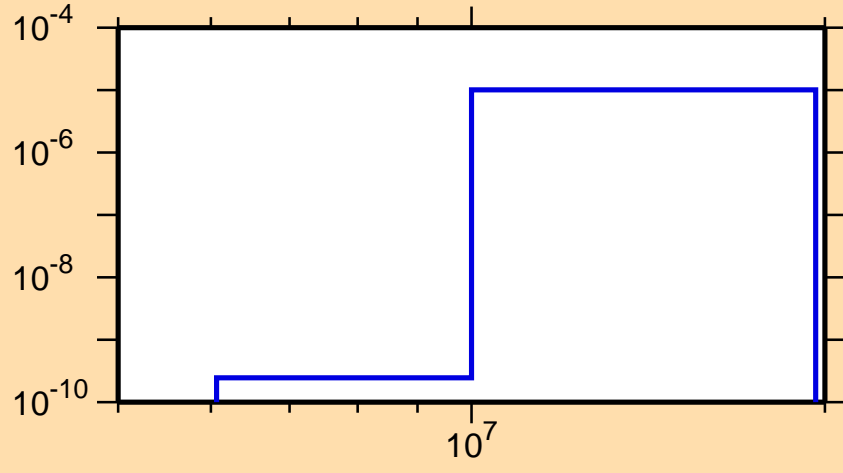
\sigma vs. E for ^{176}\text{Ir}(\text{mt } 45)
