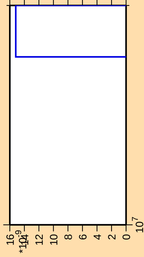
\Delta\sigma/\sigma vs. E for ^{181}\text{Ir} (mt 42)
