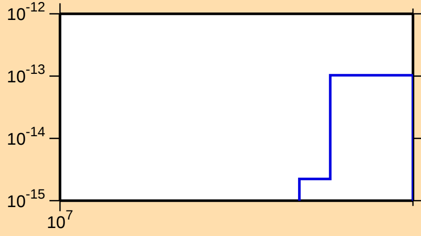
\sigma vs. E for ^{181}\text{Ir}(n,3n\alpha)
