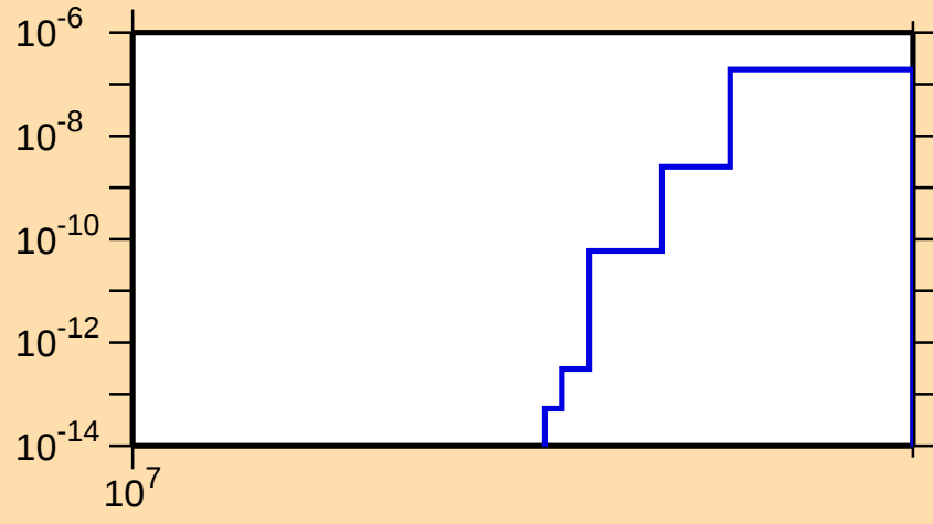
\sigma vs. E for ^{181}\text{Ir}(n,\text{nt})
