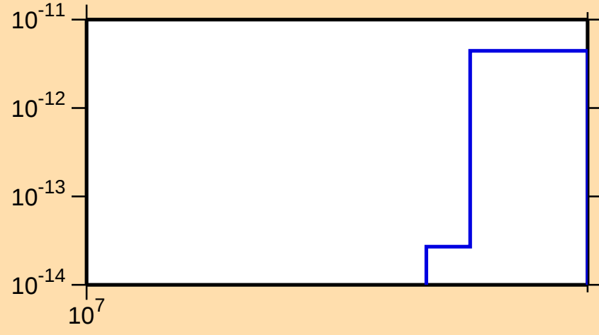
\sigma vs. E for ^{181}\text{Ir} (mt 34)
