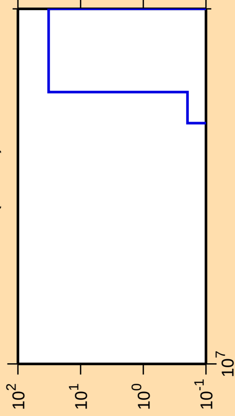
\Delta\sigma/\sigma vs. E for ^{181}\text{Ir} (mt 34)
