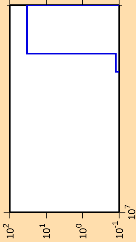
\Delta\sigma/\sigma vs. E for ^{181}\text{Ir}(n,\text{pt})
