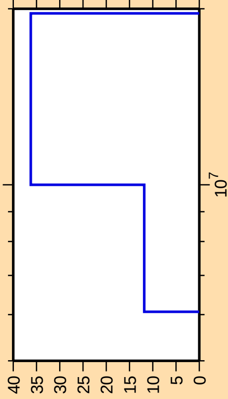
\Delta\sigma/\sigma vs. E for ^{181}\text{Ir}(n,n\text{cont.})
