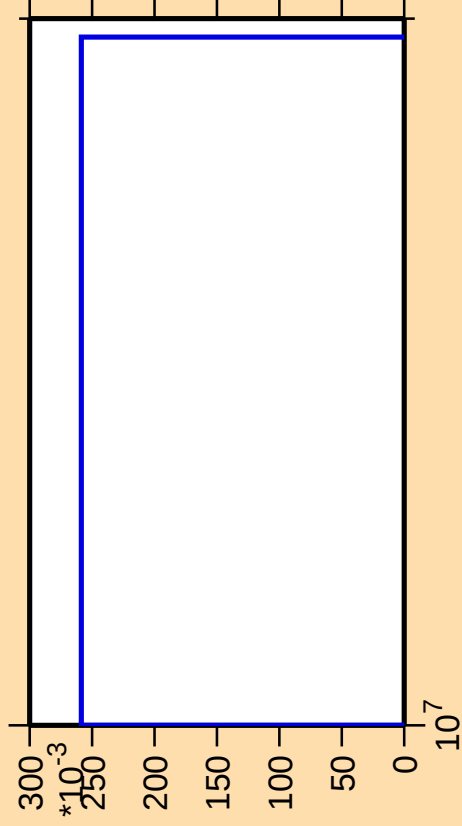
\Delta\sigma/\sigma vs. E for ^{181}\text{Ir}(n,\text{pt})
