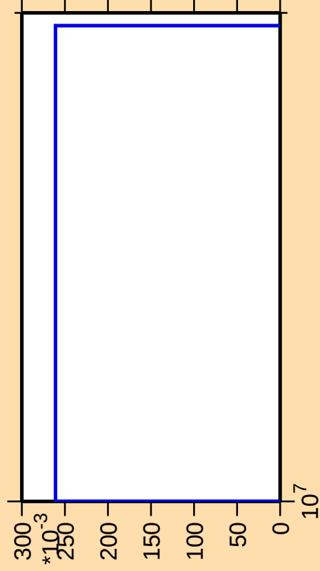
\Delta\sigma/\sigma vs. E for ^{181}\text{Ir}(\text{mt } 34)
