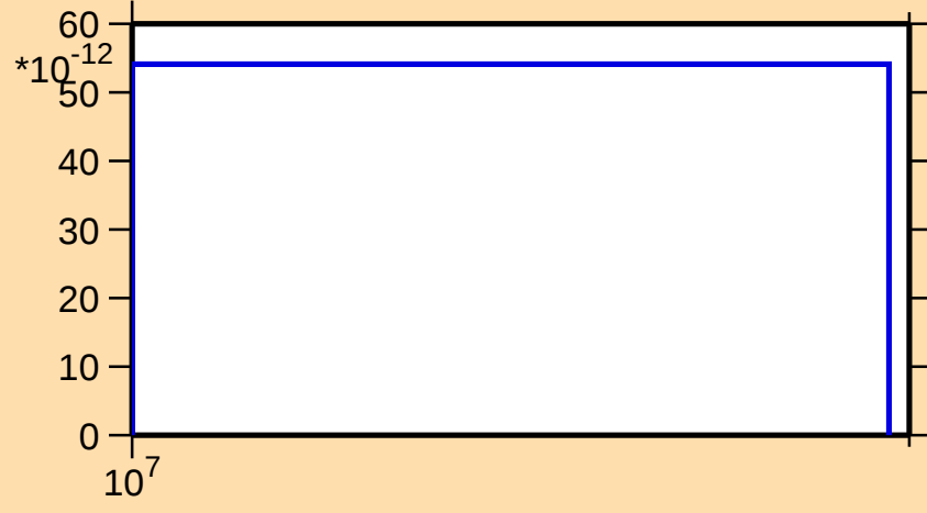
\sigma vs. E for ^{181}\text{Ir}(n,\text{pd})
