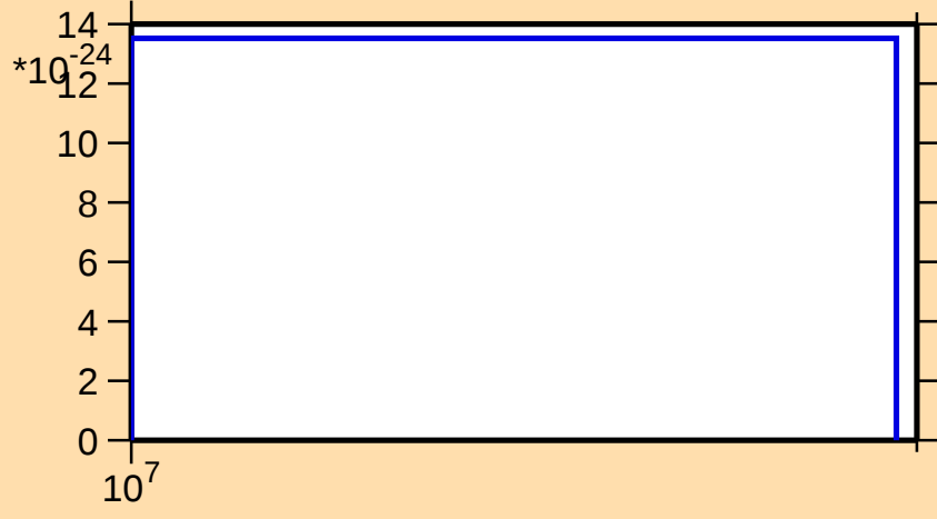
\sigma vs. E for ^{181}\text{Ir}(\text{mt } 42)
