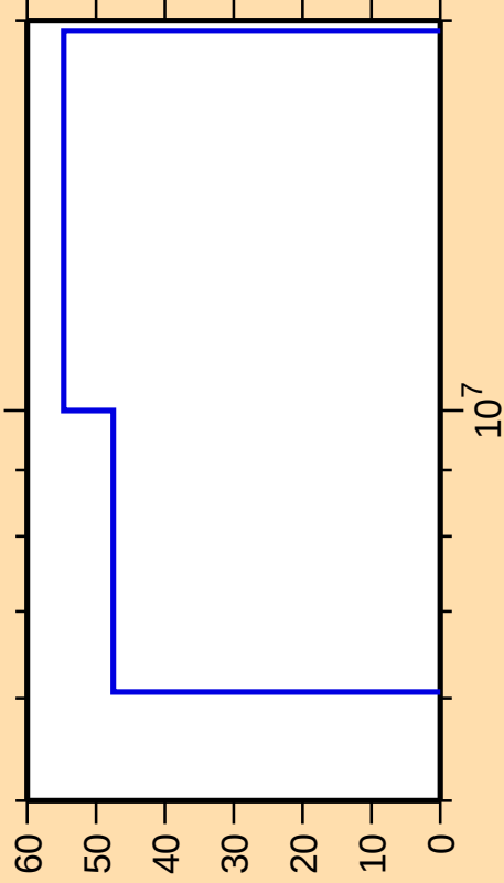
\Delta\sigma/\sigma vs. E for ^{181}\text{Ir}(n,p)
