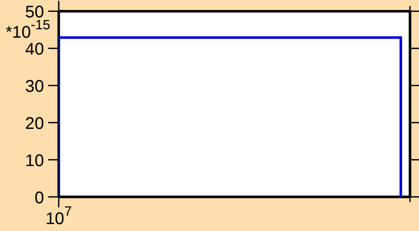
\sigma vs. E for ^{181}\text{Ir}(n,\text{pt})
