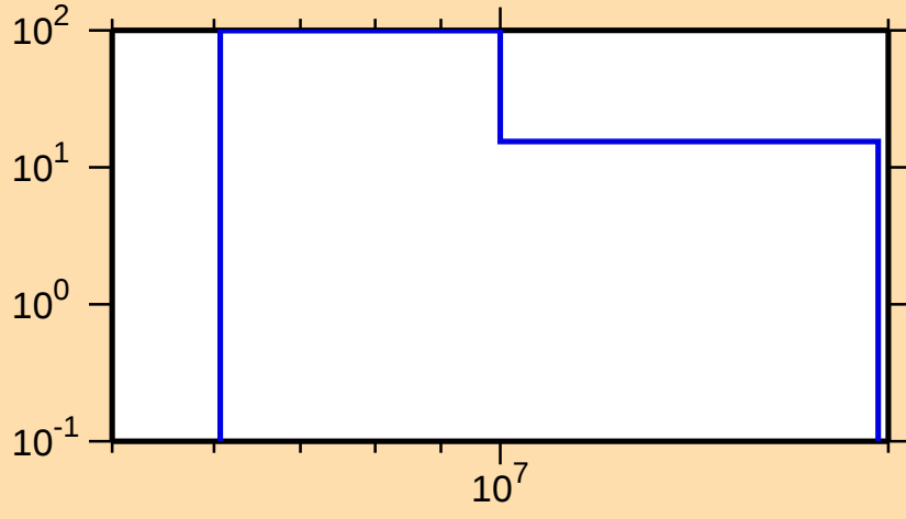
\Delta\sigma/\sigma vs. E for ^{181}\text{Ir}(n,2n)
