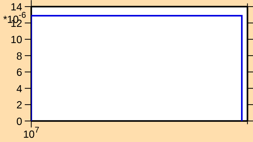
\sigma vs. E for ^{181}\text{Ir}(n,3n)
