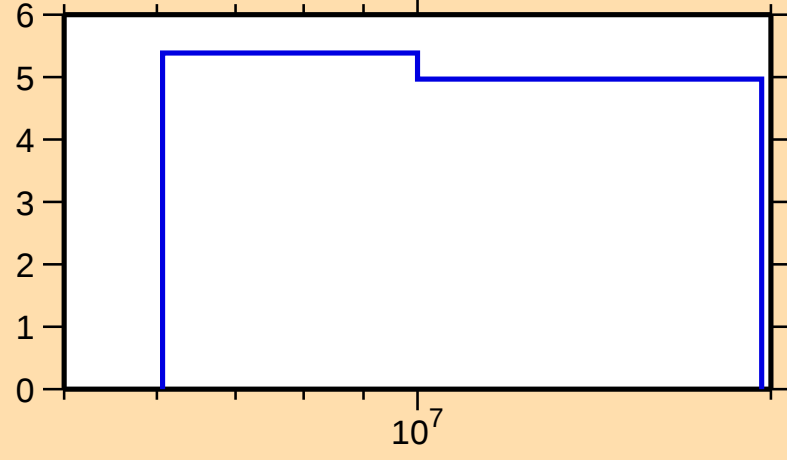
\Delta\sigma/\sigma vs. E for ^{181}\text{Ir}(n,\text{nonel.})
