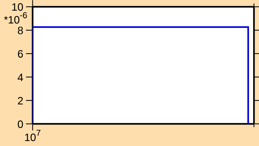
\sigma vs. E for ^{181}\text{Ir}(n,2np)
