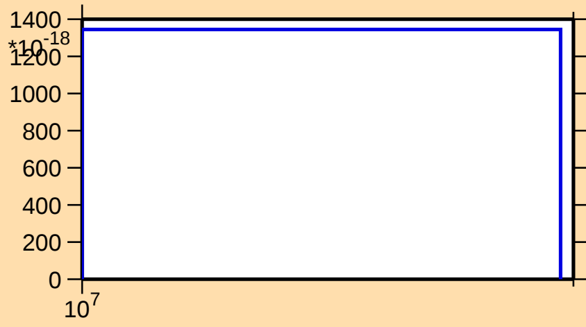
\sigma vs. E for ^{181}\text{Ir}(n,3n\alpha)
