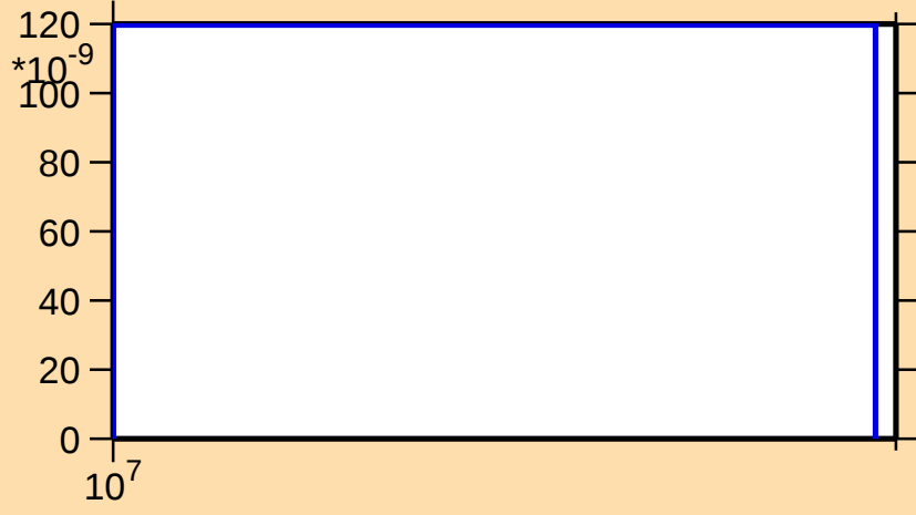
\sigma vs. E for ^{181}\text{Ir}(n,\text{nd})
