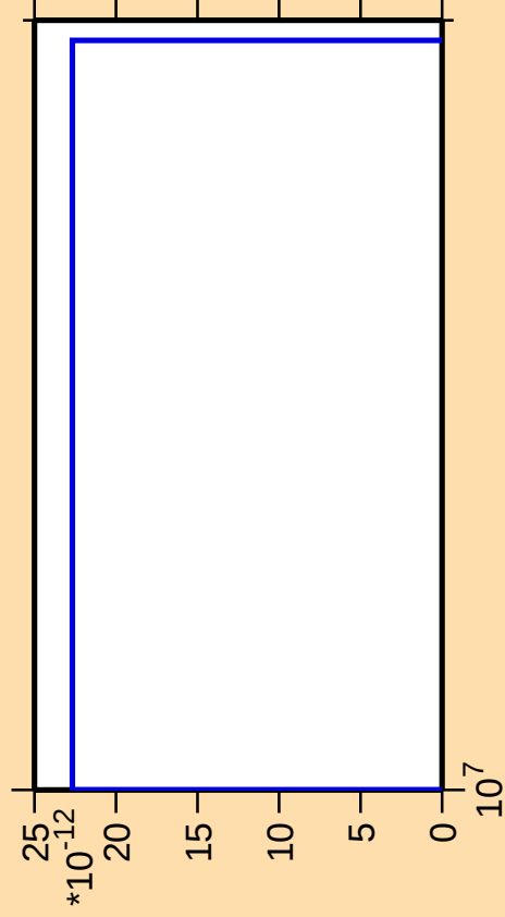
\Delta\sigma/\sigma vs. E for ^{181}\text{Ir}(\text{mt } 42)
