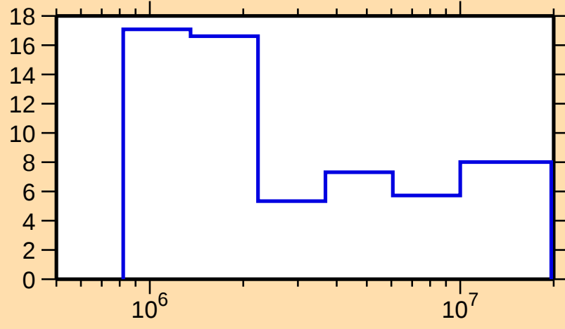
\Delta\sigma/\sigma vs. E for ^{181}\text{Ir}(n,\text{el.})
