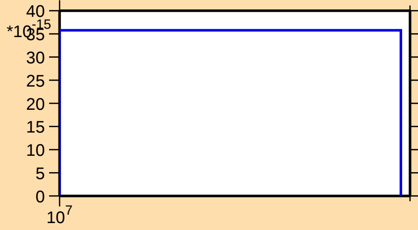
\sigma vs. E for ^{181}\text{Ir}(\text{mt } 34)
