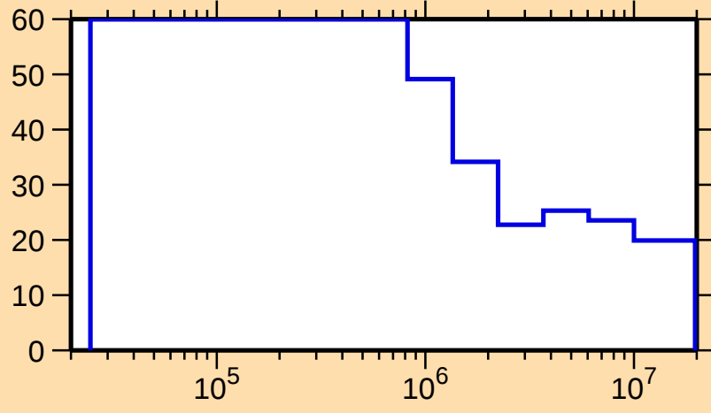
\Delta\sigma/\sigma vs. E for ^{181}\text{Ir}(n,n_1)
