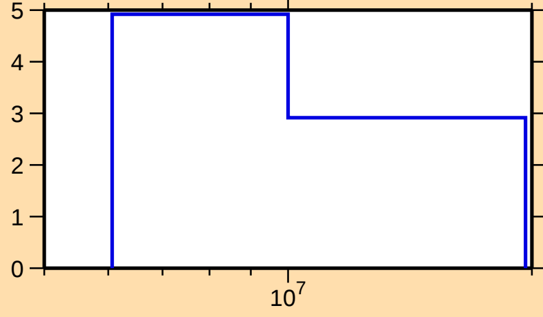
\Delta\sigma/\sigma vs. E for ^{181}\text{Ir}(n,\text{tot.})
