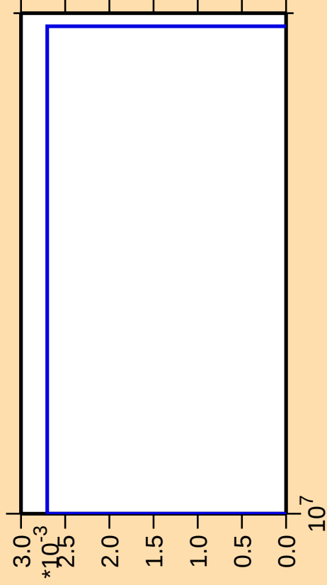
\Delta\sigma/\sigma vs. E for ^{181}\text{Ir}(n,3n\alpha)
