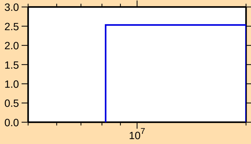
\Delta\sigma/\sigma vs. E for ^{181}\text{Ir}(n,\text{tot.})
