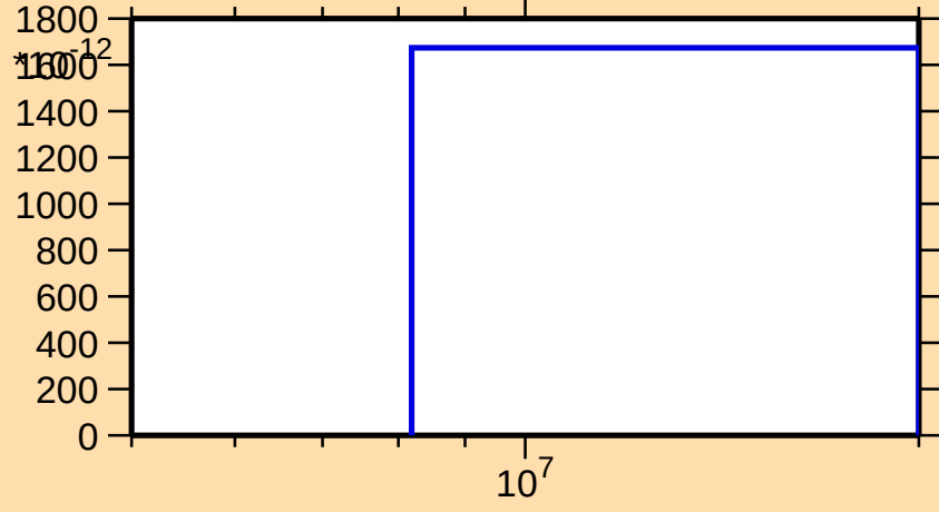
\sigma vs. E for ^{181}\text{Ir}(n,nt)
