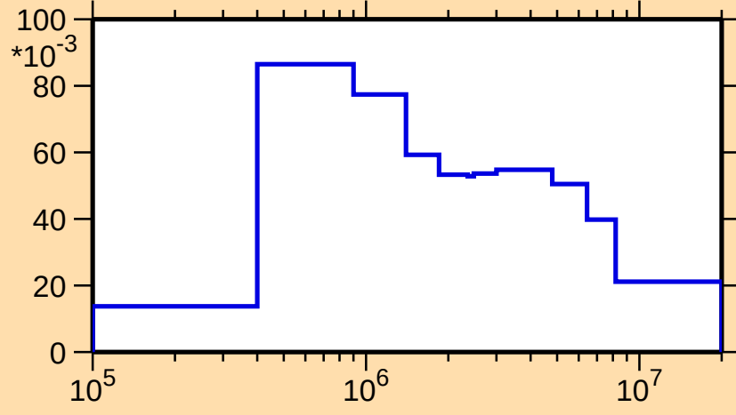
\sigma vs. E for ^{181}\text{Ir}(n,n_4)
