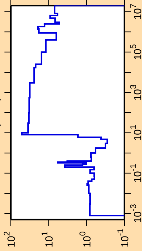
\Delta\sigma/\sigma vs. E for ^{181}\text{Ir}(n,\text{el.})
