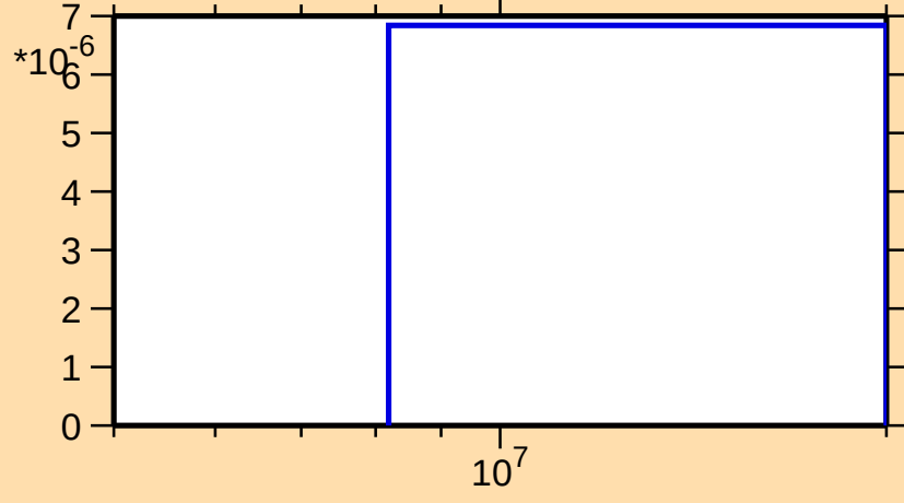
\sigma vs. E for ^{181}\text{Ir}(n,2np)
