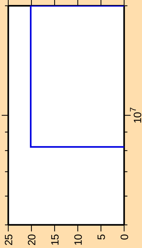
\Delta\sigma/\sigma vs. E for ^{181}\text{Ir}(n,n_1)
