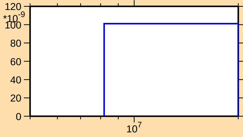
\sigma vs. E for ^{181}\text{Ir}(n,\text{He3})
