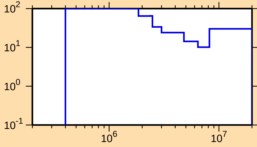
\Delta\sigma/\sigma vs. E for ^{181}\text{Ir}(n,n\text{cont.})
