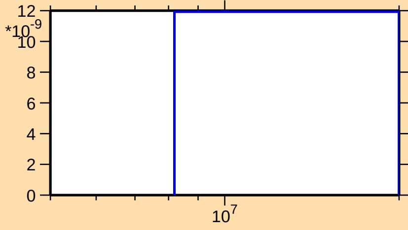
\sigma vs. E for ^{181}\text{Ir}(\text{mt } 45)
