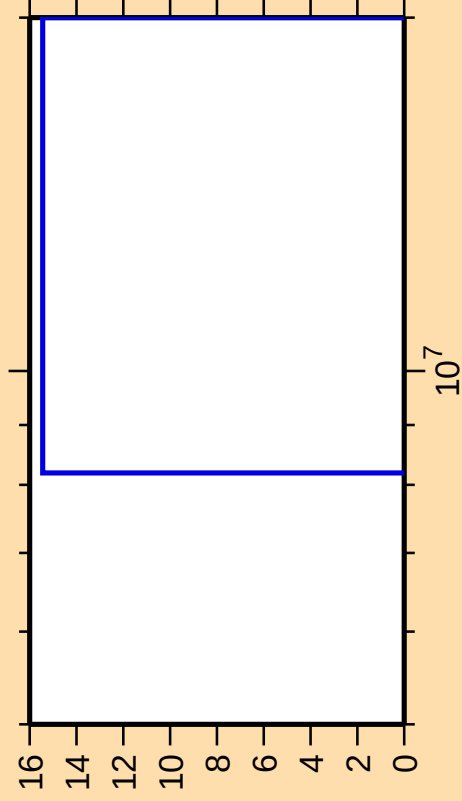
\Delta\sigma/\sigma vs. E for ^{181}\text{Ir}(n,2n)
