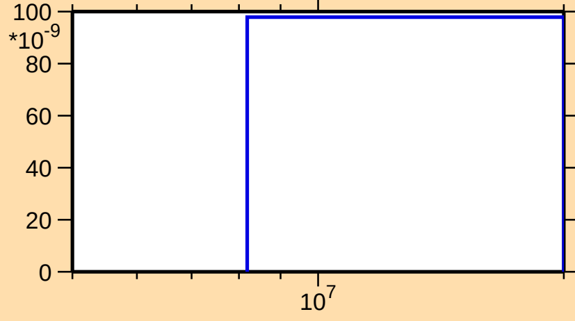
\sigma vs. E for ^{181}\text{Ir}(n,2n\alpha)
