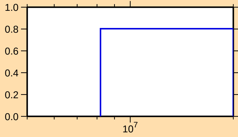
\sigma vs. E for ^{181}\text{Ir}(n,2n)
