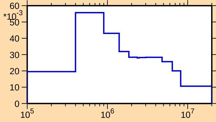
\sigma vs. E for ^{181}\text{Ir}(n,n_2)
