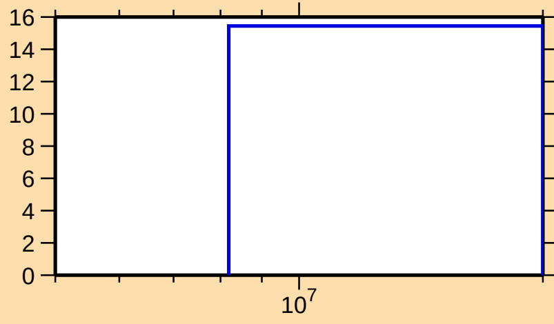
\Delta\sigma/\sigma vs. E for ^{181}\text{Ir}(n,2n)
