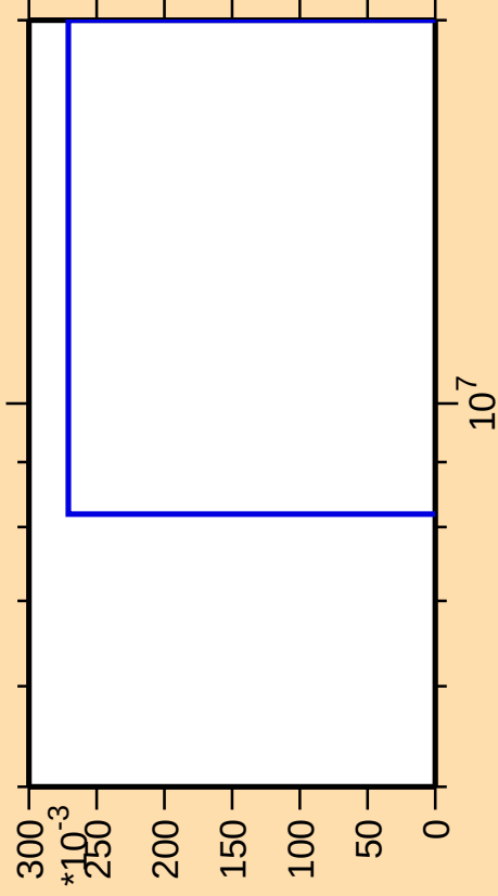
\Delta\sigma/\sigma vs. E for ^{181}\text{Ir}(\text{mt } 34)
