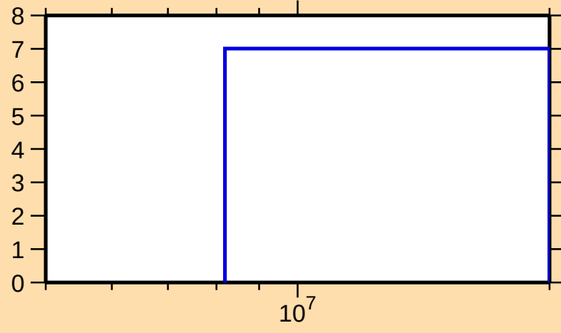
\Delta\sigma/\sigma vs. E for ^{181}\text{Ir}(n,\text{el.})
