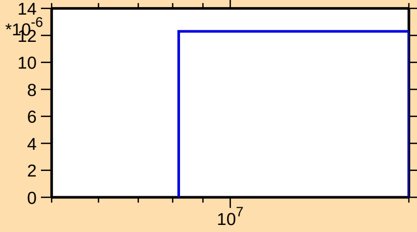
\sigma vs. E for ^{181}\text{Ir}(n,3n)
