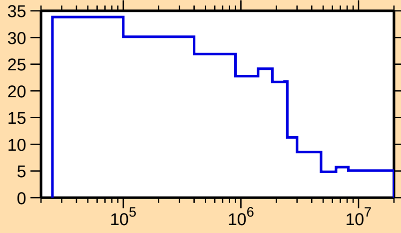
\Delta\sigma/\sigma vs. E for ^{181}\text{Ir}(n,\text{nonel.})
