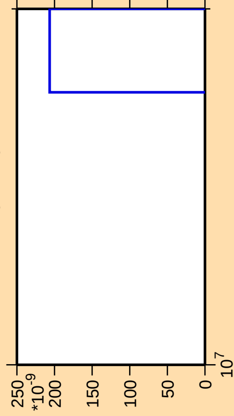
\Delta\sigma/\sigma vs. E for ^{184}\text{Ir}(\text{mt } 42)
