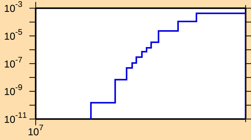
\sigma vs. E for ^{184}\text{Ir}(n,2np)
