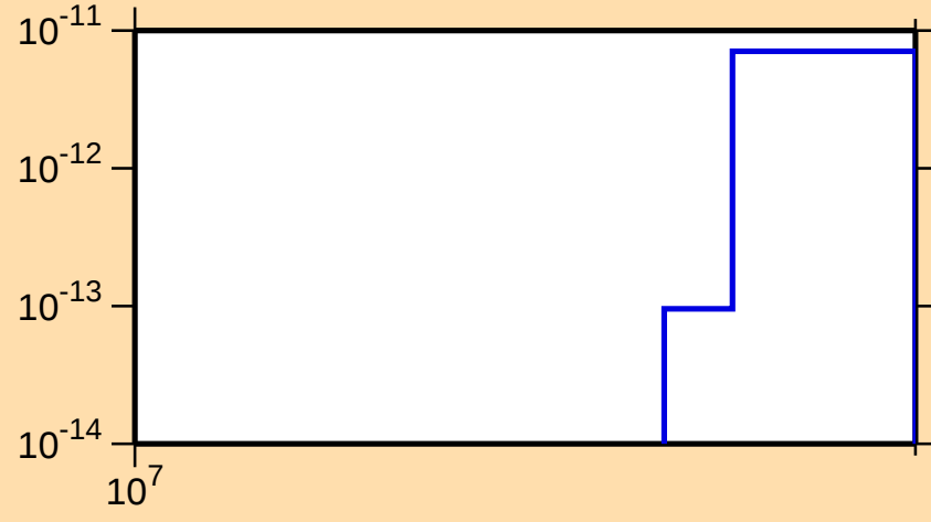
\sigma vs. E for ^{184}\text{Ir}(n,\text{pt})
