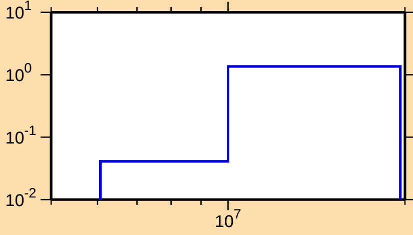
\sigma vs. E for ^{184}\text{Ir}(n,2n)
