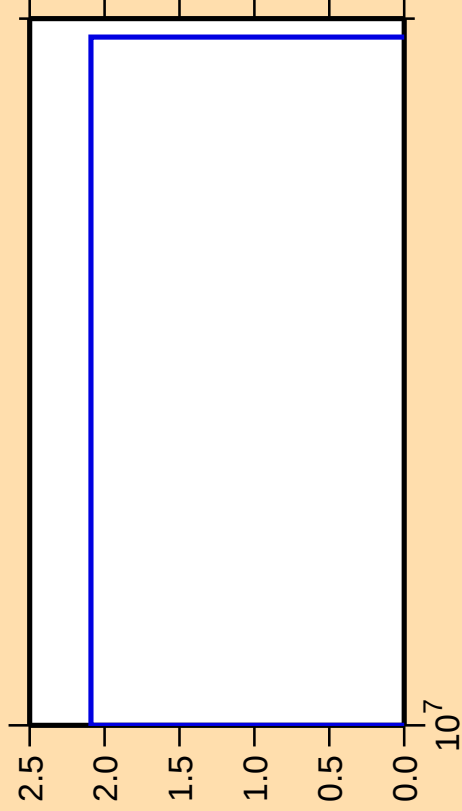
\Delta\sigma/\sigma vs. E for ^{184}\text{Ir}(n,\text{pd})
