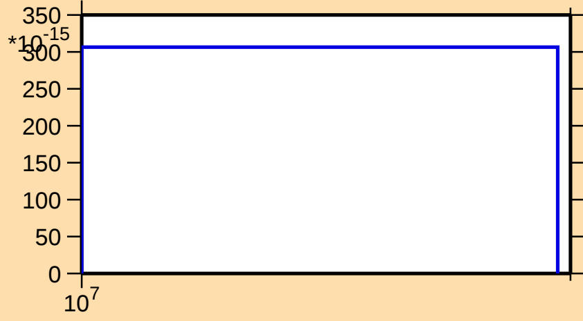
\sigma vs. E for ^{184}\text{Ir}(n,\text{pd})
