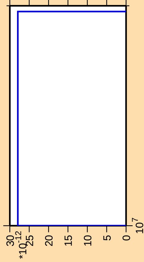
\Delta\sigma/\sigma vs. E for ^{184}\text{Ir}(\text{mt } 42)
