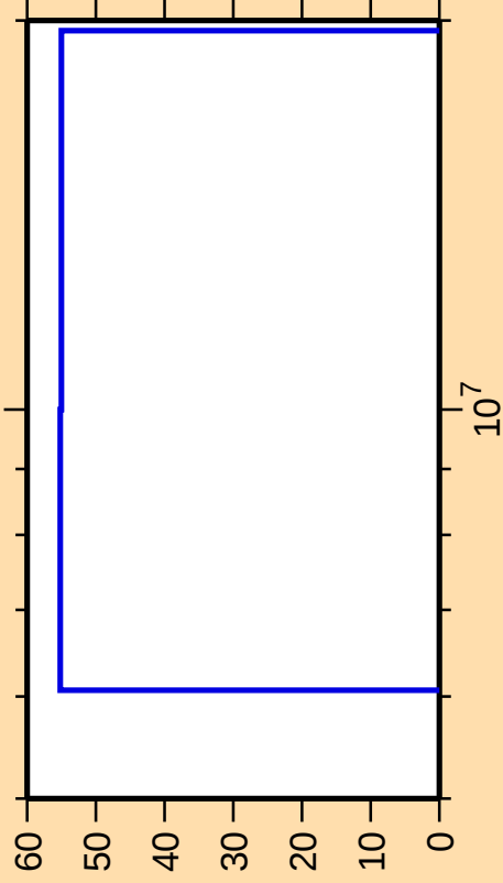
\Delta\sigma/\sigma vs. E for ^{184}\text{Ir}(n,p)
