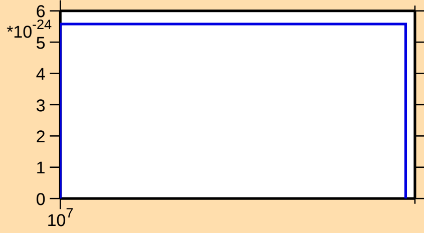
\sigma vs. E for ^{184}\text{Ir}(\text{mt } 42)
