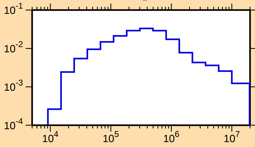
\sigma vs. E for ^{184}\text{Ir}(n,n_1)
