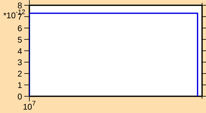
\sigma vs. E for ^{184}\text{Ir}(\text{mt117})
