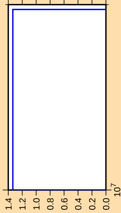
\Delta\sigma/\sigma vs. E for ^{184}\text{Ir}(\text{mt } 34)
