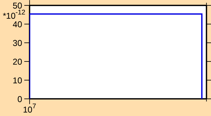
\sigma vs. E for ^{184}\text{Ir}(\text{mt 45})
