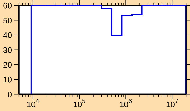
\Delta\sigma/\sigma vs. E for ^{184}\text{Ir}(n,n_1)
