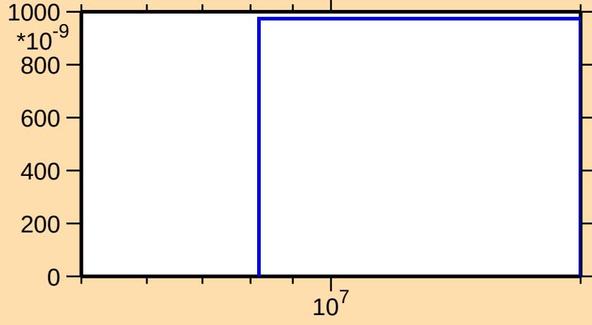
\sigma vs. E for ^{184}\text{Ir}(n,2n\alpha)
