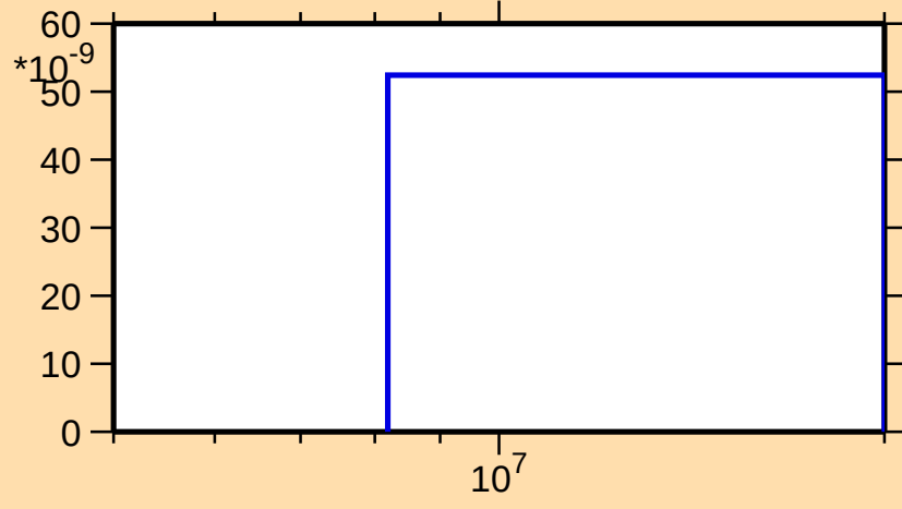
\sigma vs. E for ^{184}\text{Ir}(n,\text{He3})
