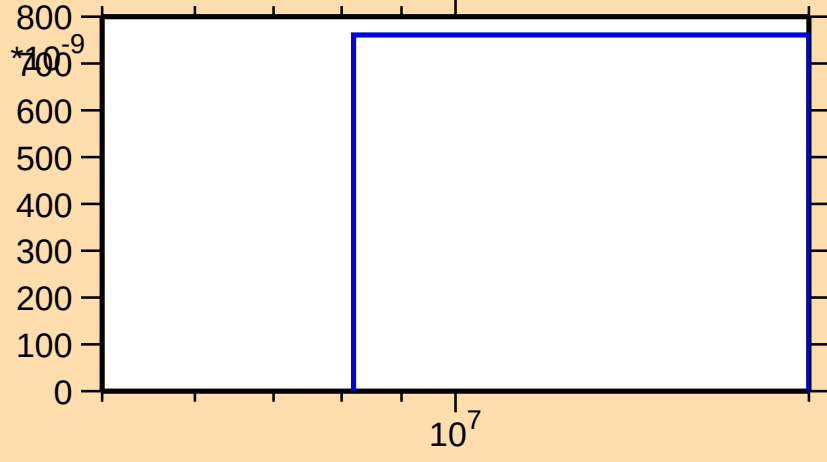
\sigma vs. E for ^{184}\text{Ir}(n,\text{nd})
