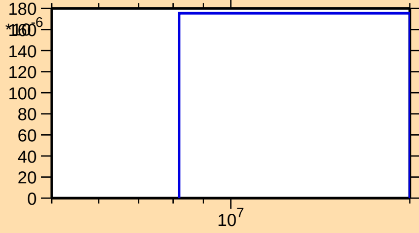
\sigma vs. E for ^{184}\text{Ir}(n,3n)
