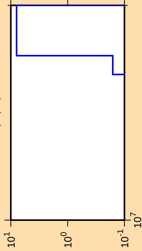
\Delta\sigma/\sigma vs. E for ^{186}\text{Ir}(n,\text{pd})
