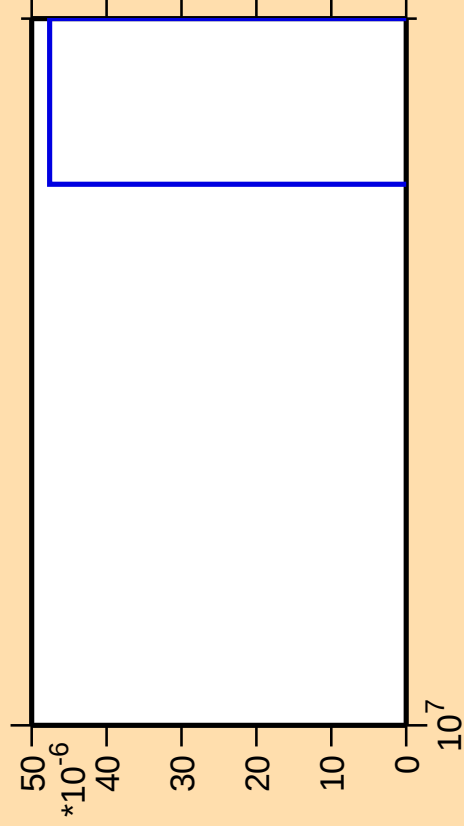
\Delta\sigma/\sigma vs. E for ^{186}\text{Ir}(\text{mt } 42)
