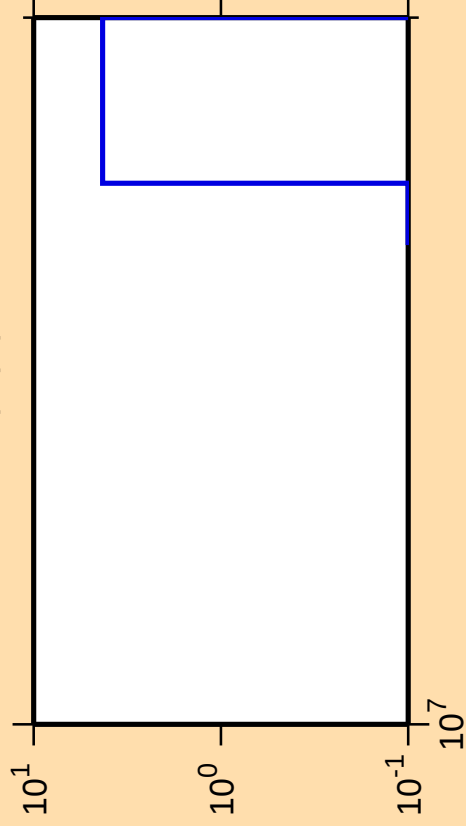
\Delta\sigma/\sigma vs. E for ^{186}\text{Ir}(n,\text{pt})
