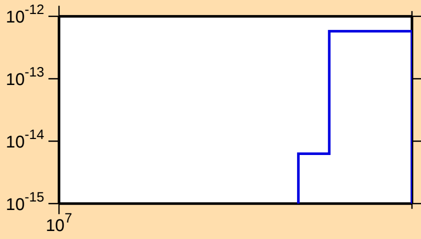
\sigma vs. E for ^{186}\text{Ir}(n,\text{pt})
