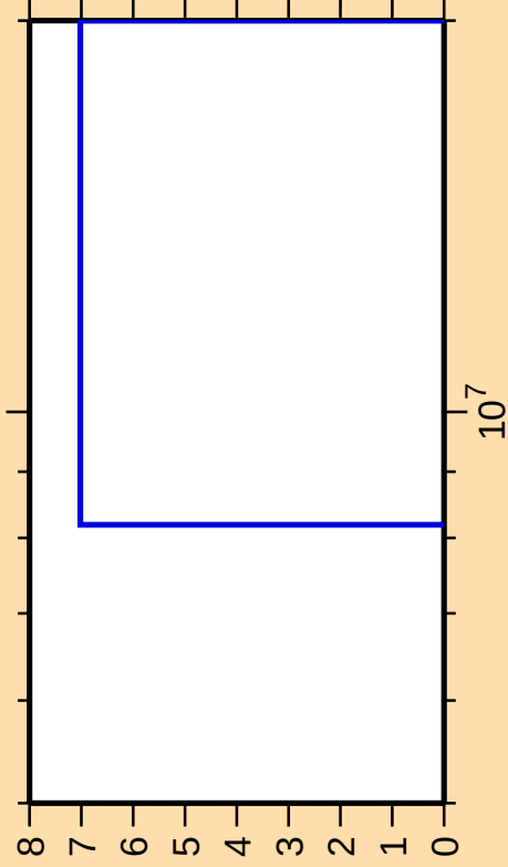
\Delta\sigma/\sigma vs. E for ^{186}\text{Ir}(\text{mt } 45)
