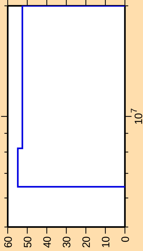
\Delta\sigma/\sigma vs. E for ^{186}\text{Ir}(n,n_1)
