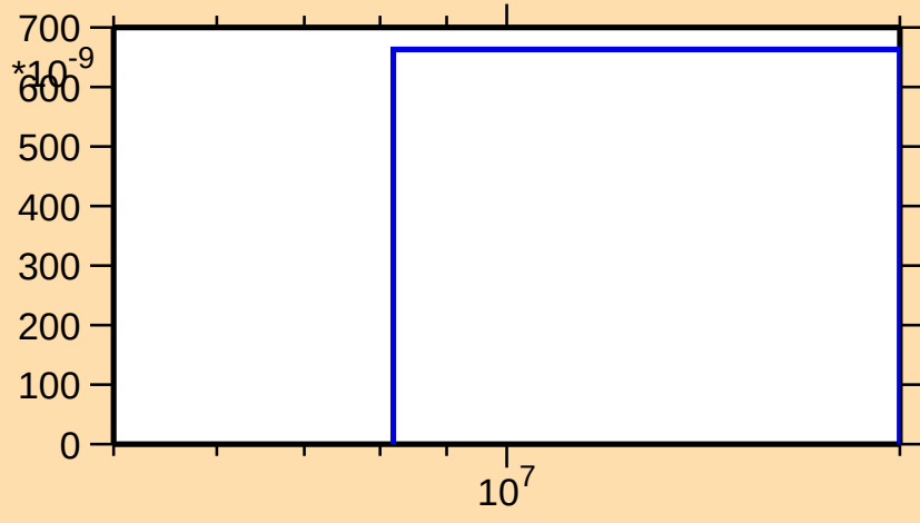
\sigma vs. E for ^{186}\text{Ir}(n,2n\alpha)
