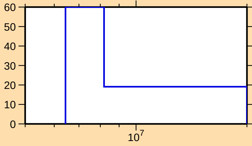
\Delta\sigma/\sigma vs. E for ^{186}\text{Ir}(n,2n)
