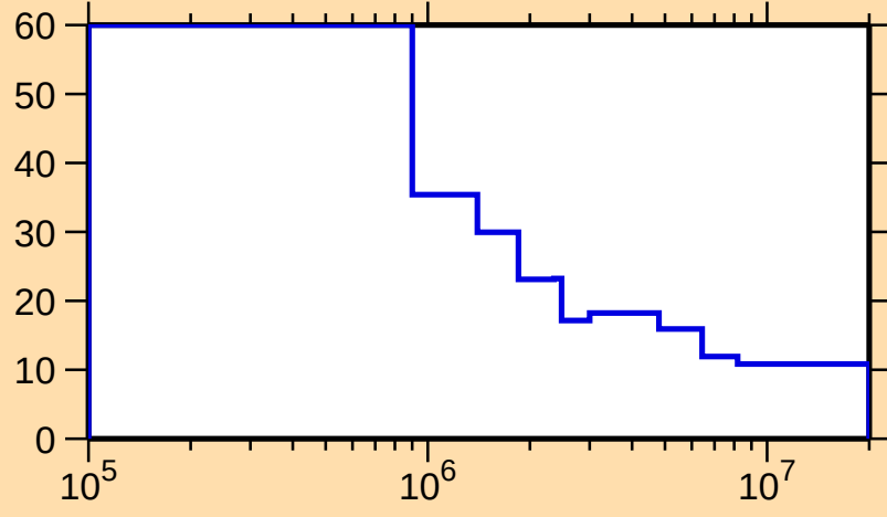
\Delta\sigma/\sigma vs. E for ^{186}\text{Ir}(n,\text{nonel.})
